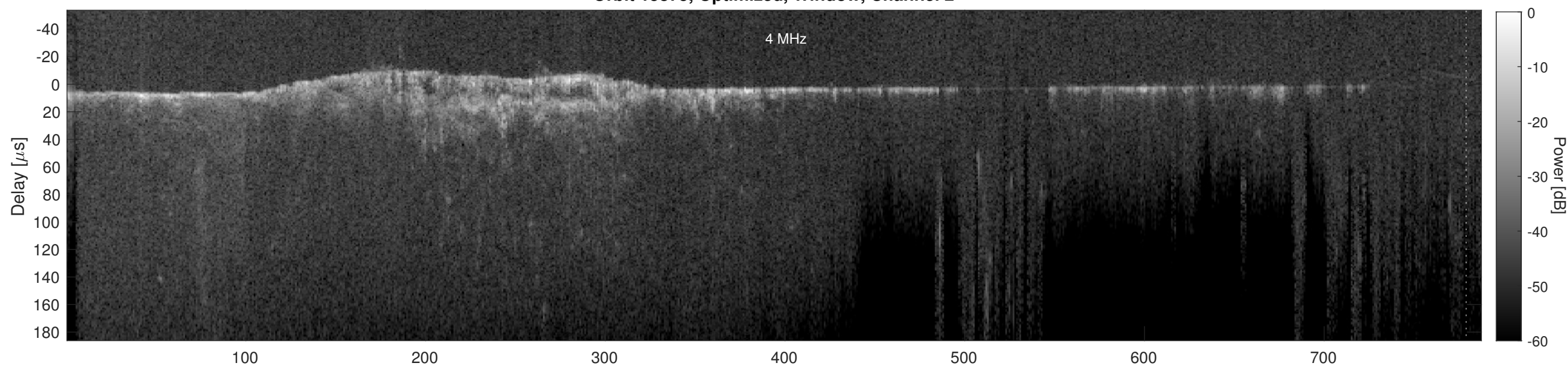
Orbit 15875, Cluttergram
