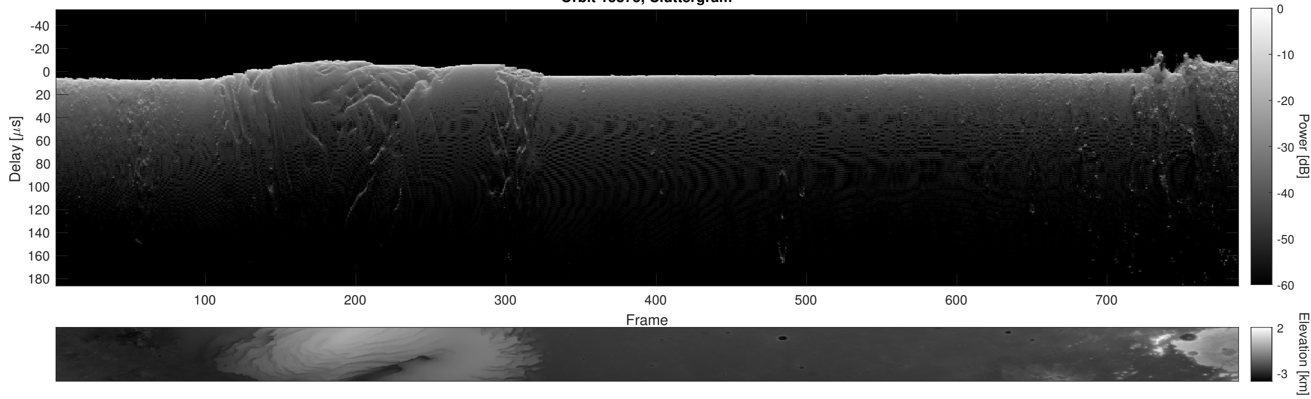
Orbit 15875, Cluttergram
