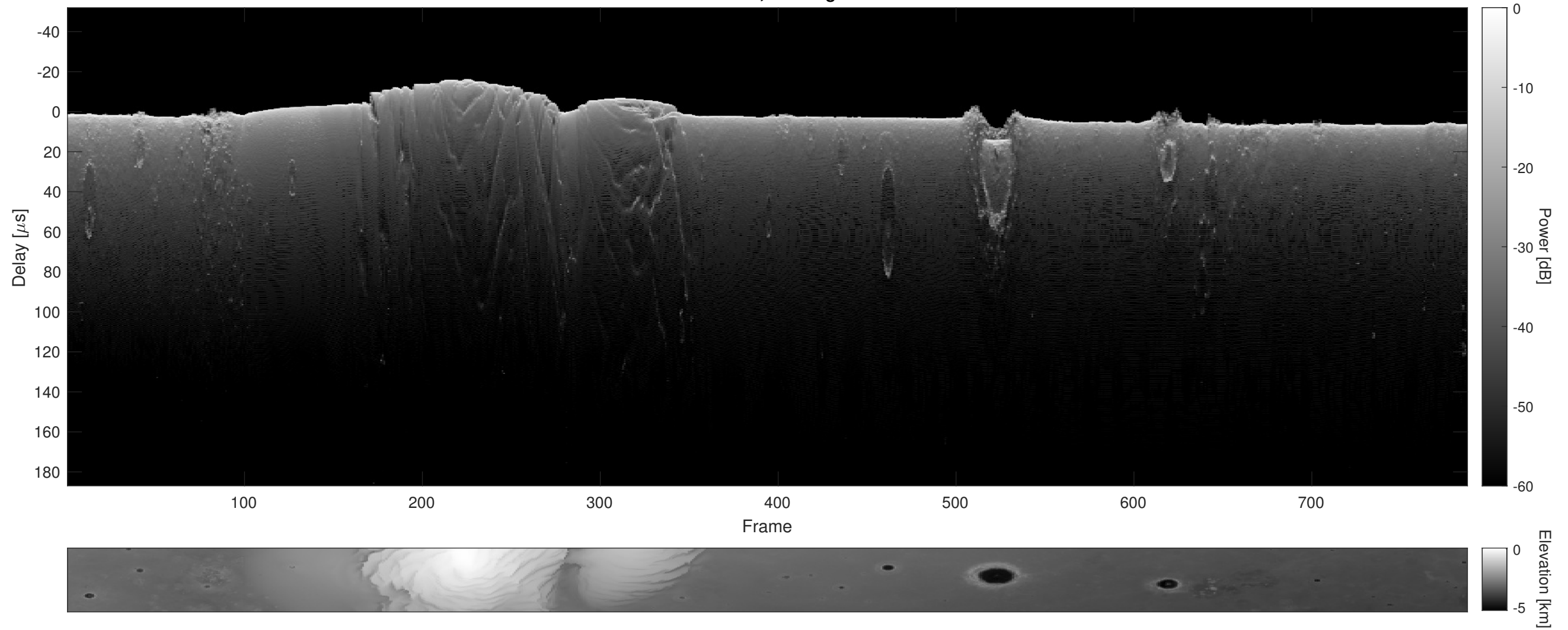
Orbit 15886, Cluttergram
