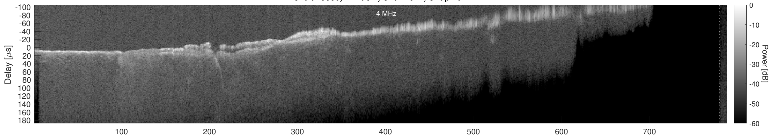
Orbit 15886, Window, Channel 2, Optimized
