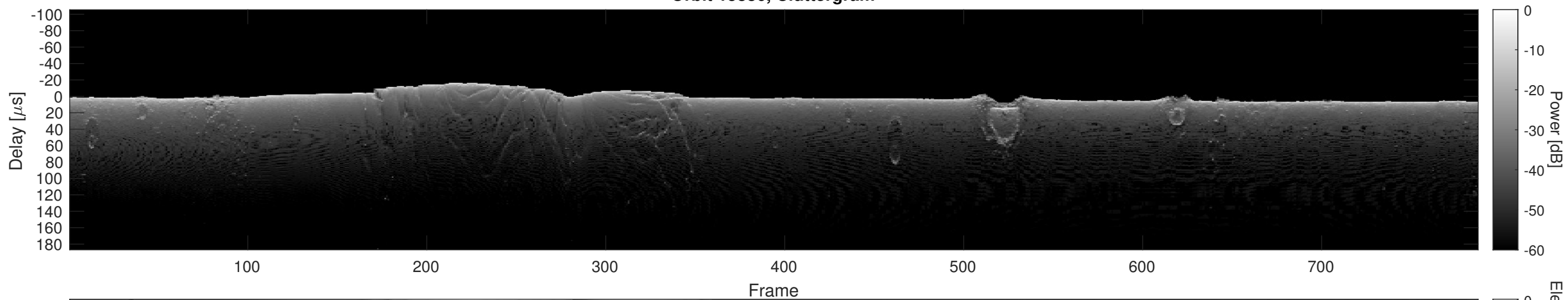
Orbit 15886, Cluttergram
