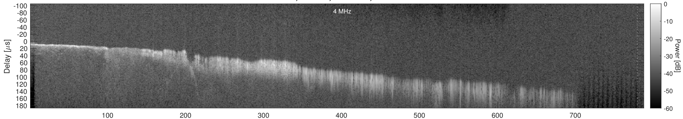
Orbit 15886, Window, Channel 2, Chapman
