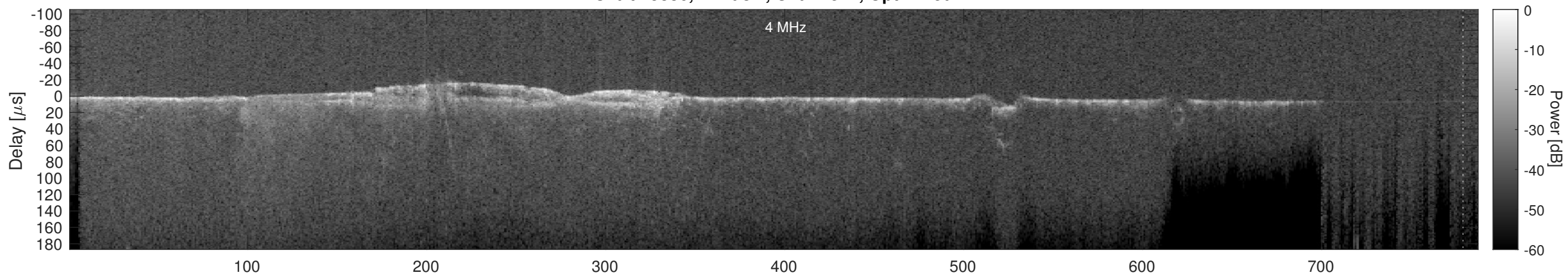
Orbit 15886, Cluttergram
