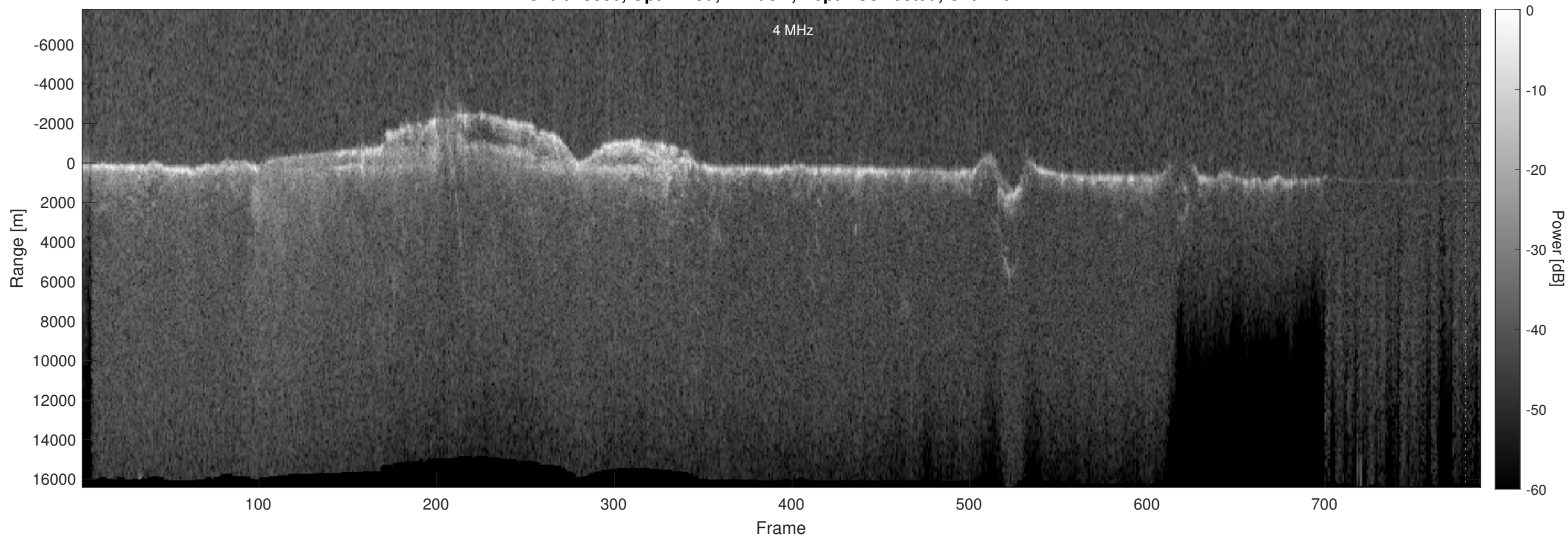
Orbit 15886, Optimized, Window, Depth-Corrected, Channel 2
