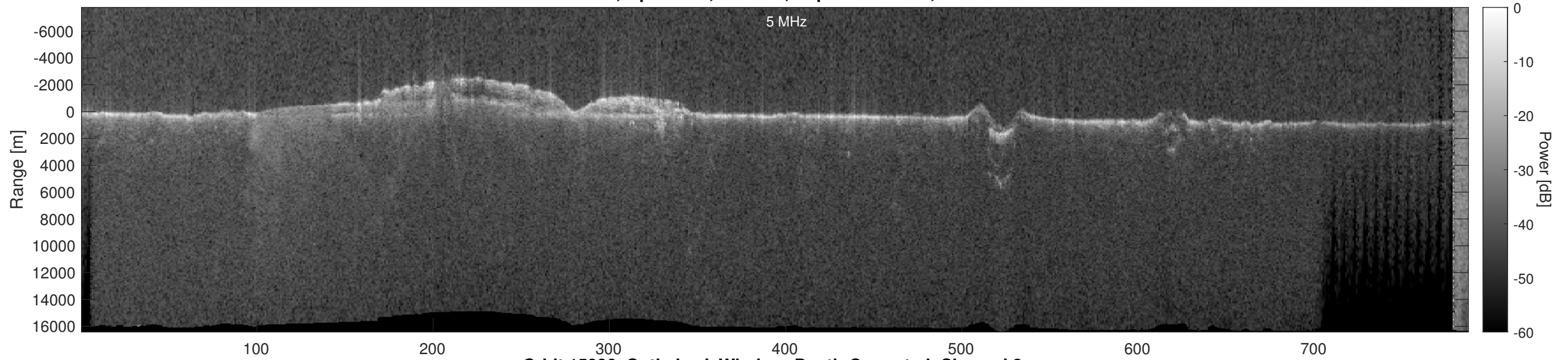
Orbit 15886, Optimized, Window, Depth-Corrected, Channel 2
