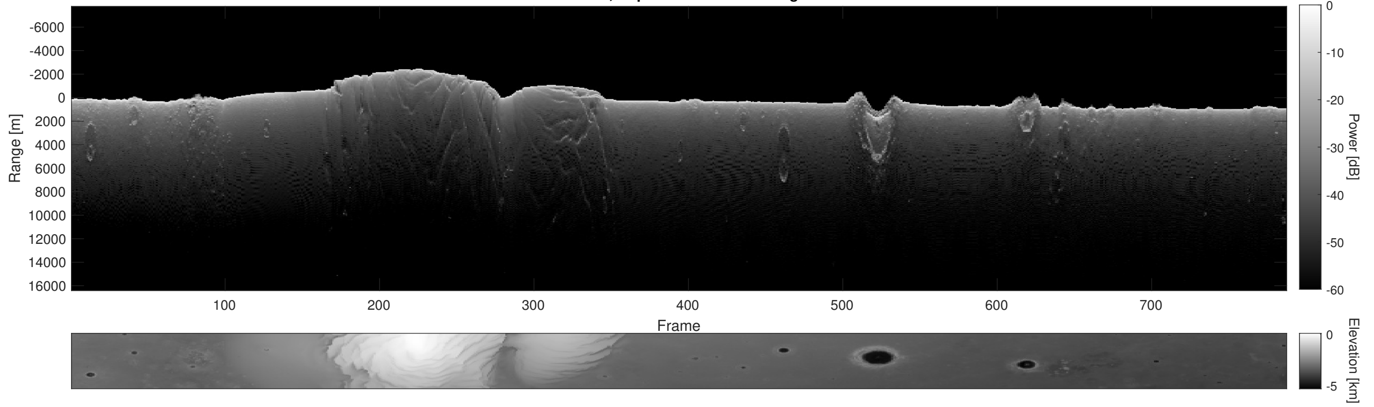
Orbit 15886, Depth-Corrected Cluttergram
