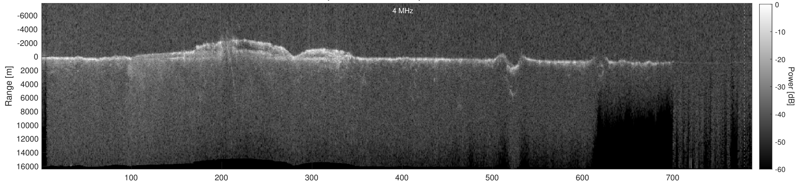
Orbit 15886, Depth-Corrected Cluttergram
