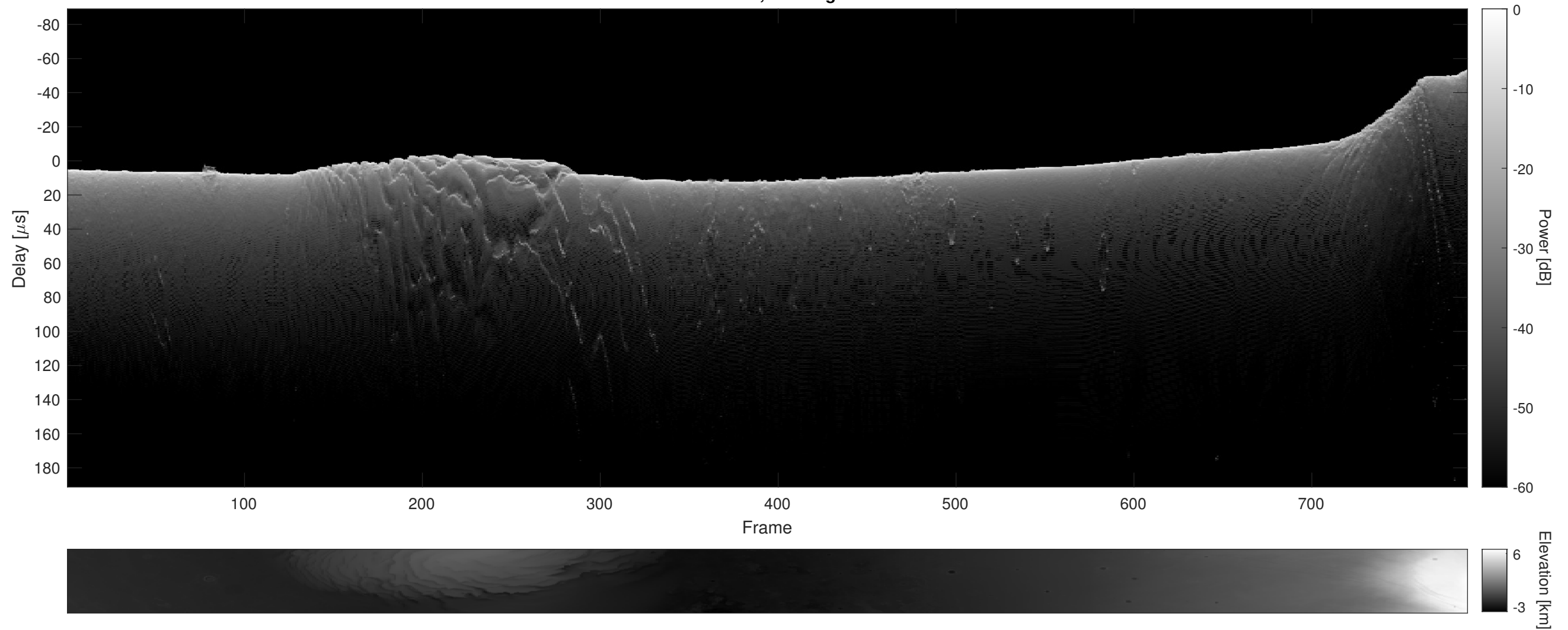
Orbit 15887, Cluttergram
