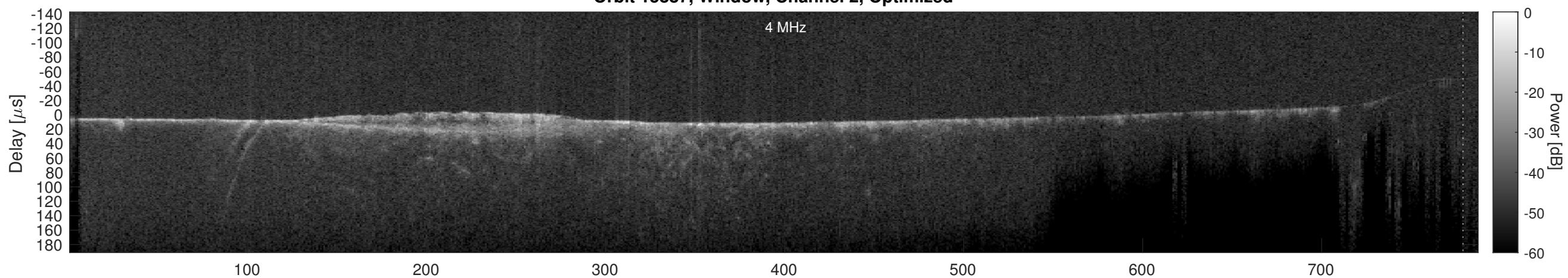
Orbit 15887, Cluttergram
