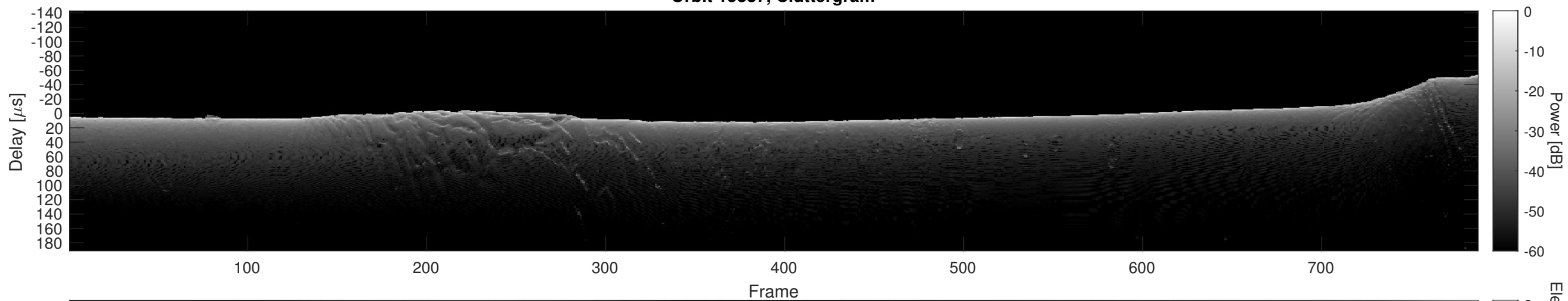
Orbit 15887, Cluttergram
