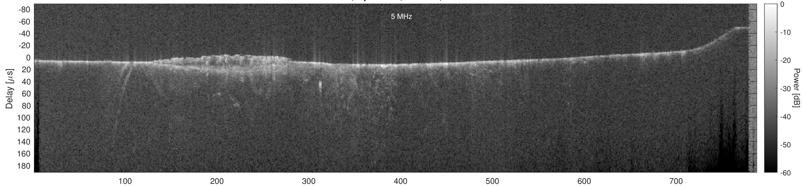
Orbit 15887, Optimized, Window, Channel 2
