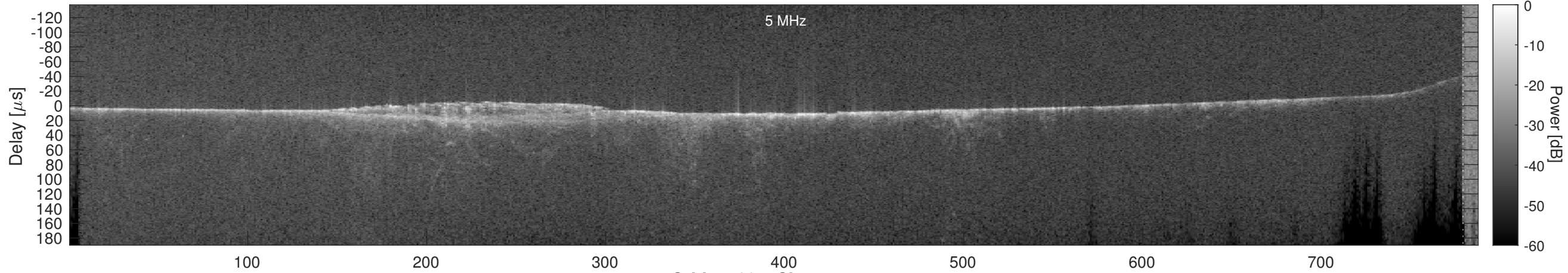
Orbit 15894, Cluttergram
