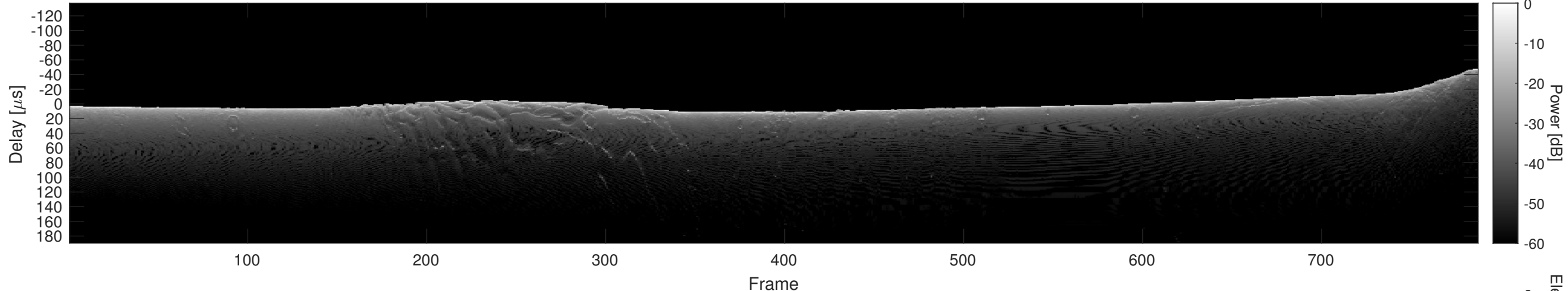
Orbit 15894, Cluttergram
