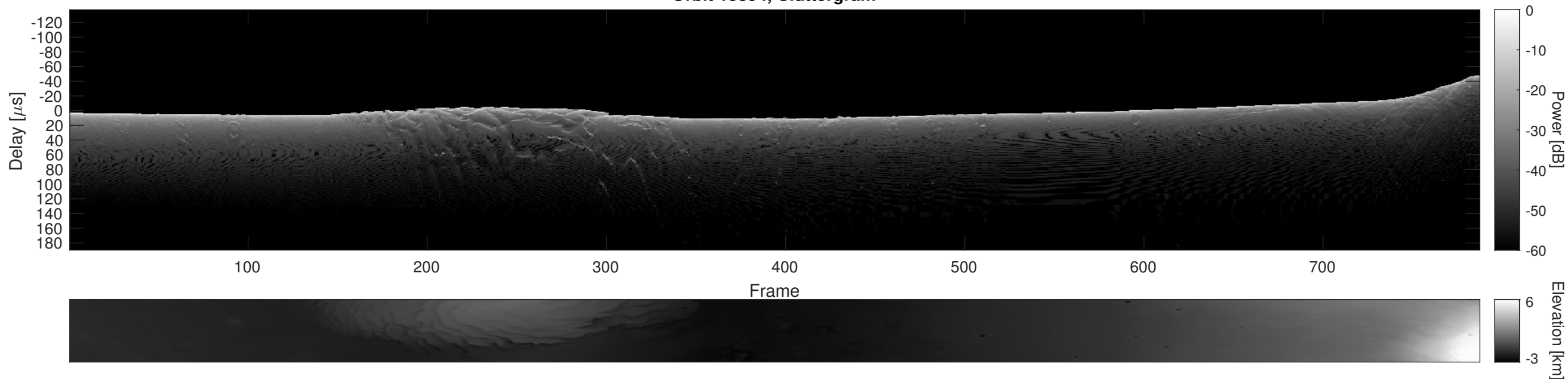
Orbit 15894, Cluttergram
