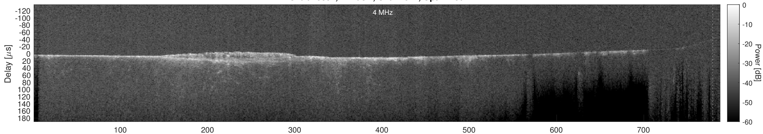
Orbit 15894, Cluttergram
