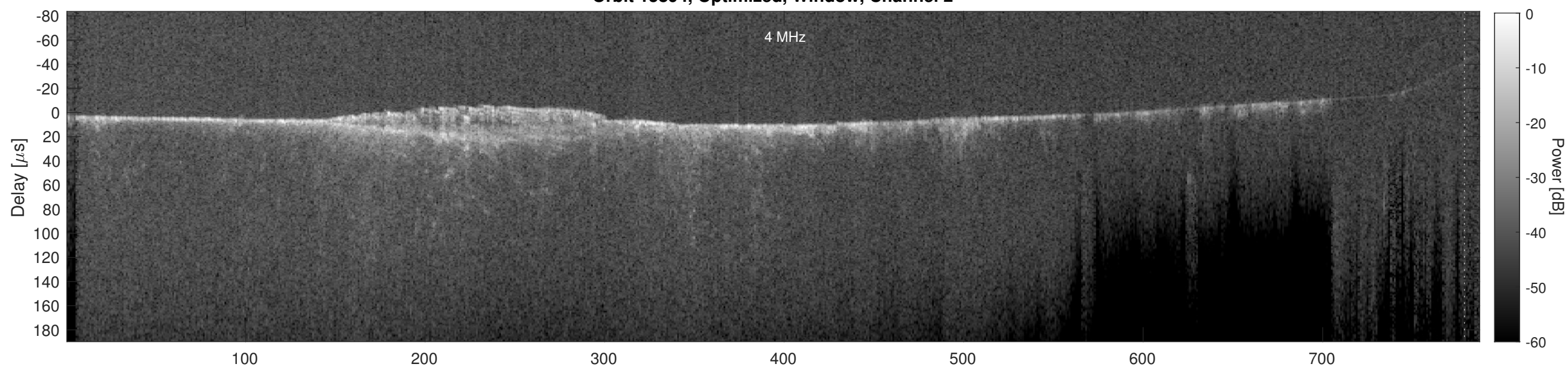
Orbit 15894, Cluttergram
