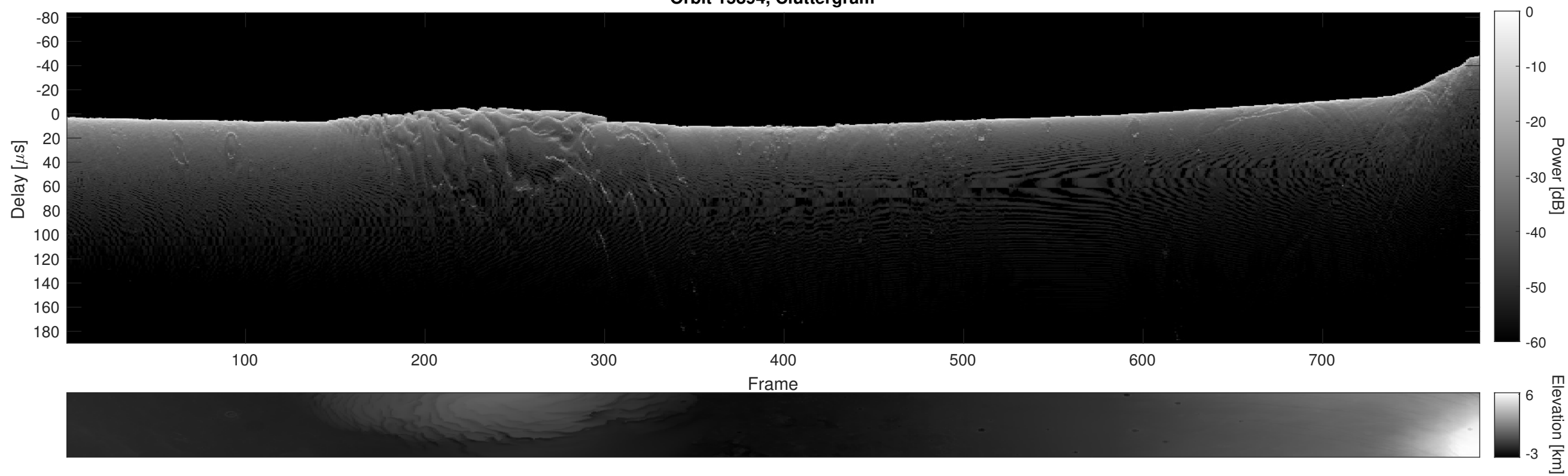
Orbit 15894, Cluttergram
