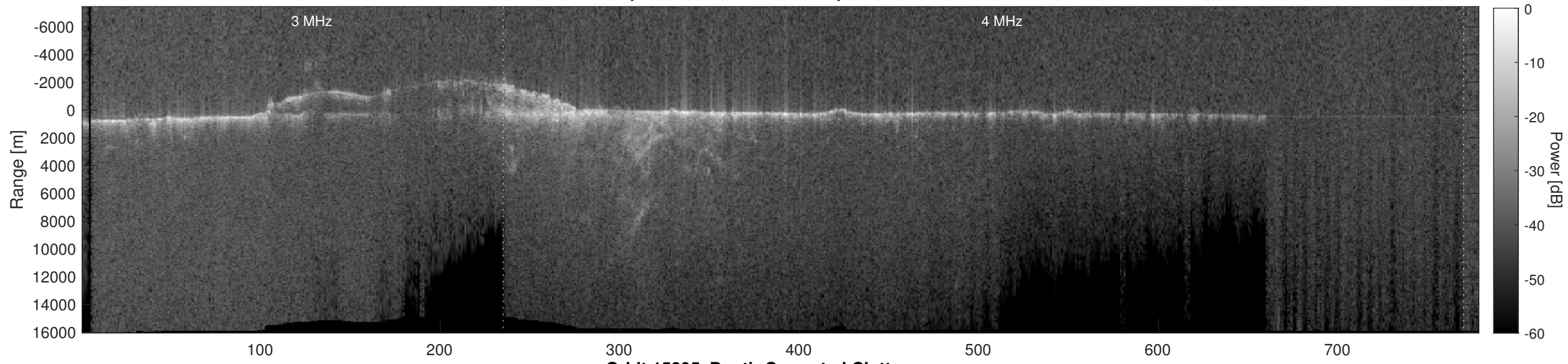
Orbit 15895, Depth-Corrected Cluttergram
