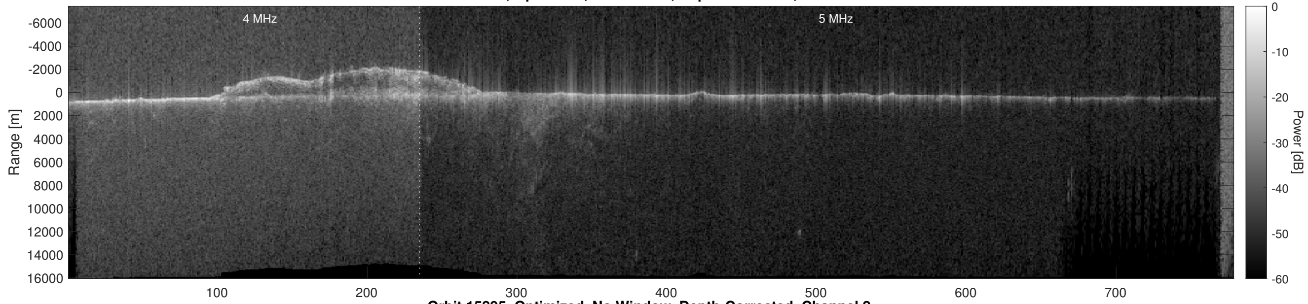
Orbit 15895, Optimized, No Window, Depth-Corrected, Channel 2
