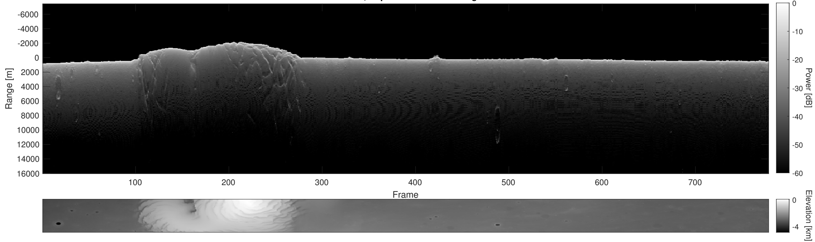
Orbit 15895, Depth-Corrected Cluttergram
