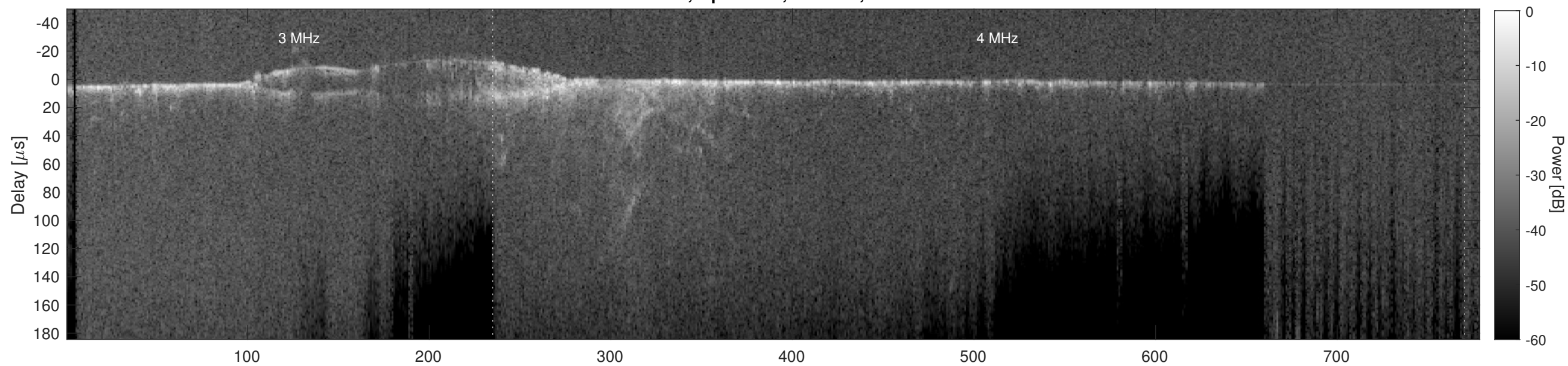
Orbit 15895, Cluttergram
