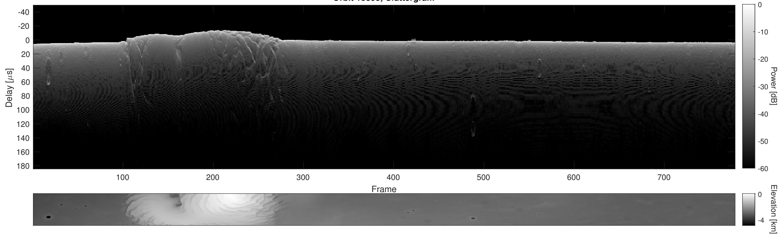
Orbit 15895, Cluttergram
