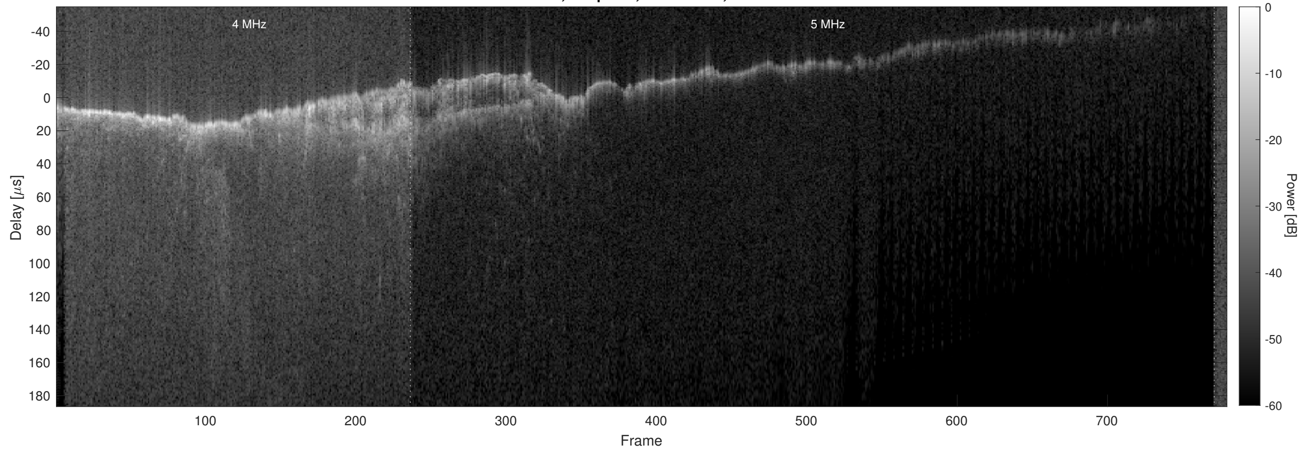
Orbit 15896, Chapman, No Window, Channel 2
