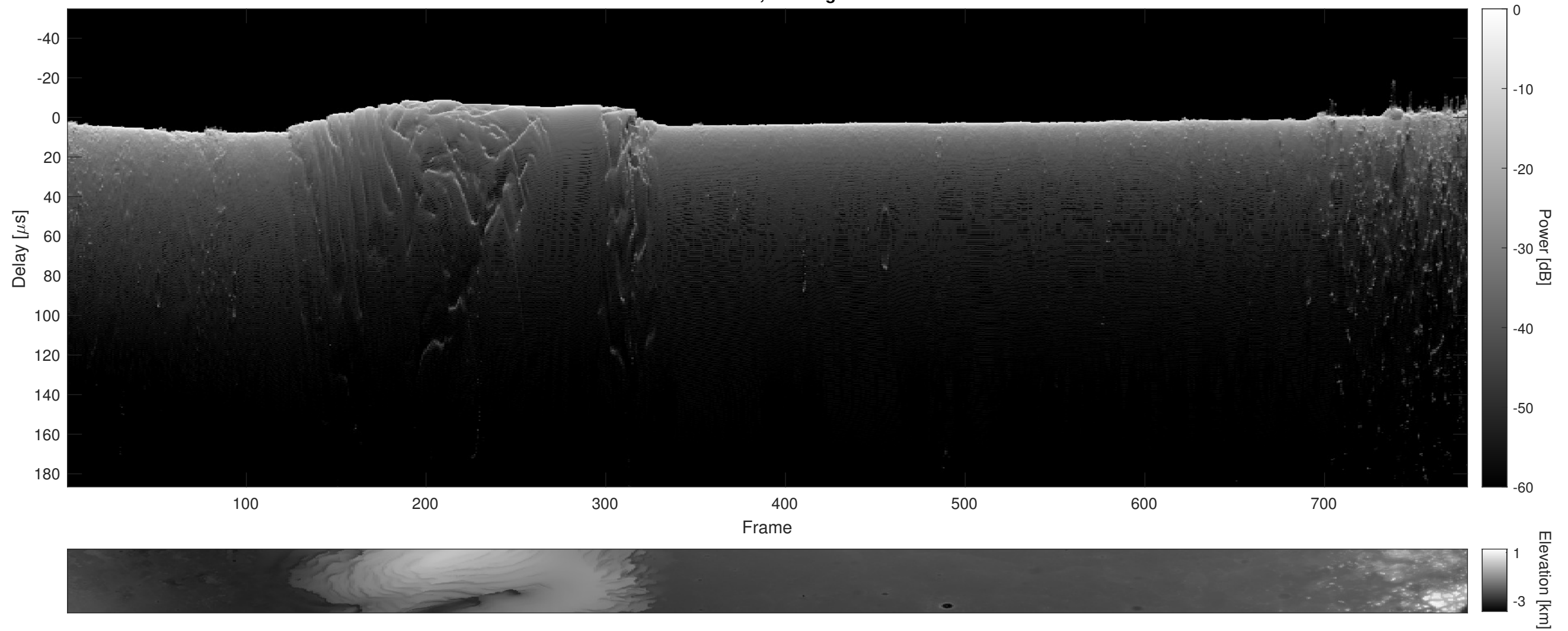
Orbit 15896, Cluttergram
