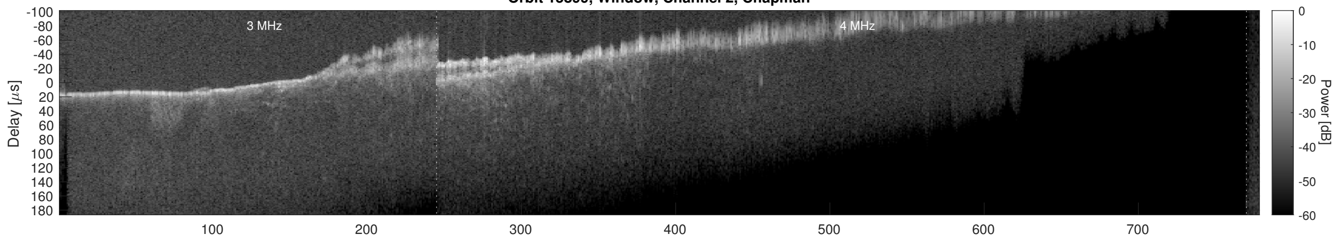
Orbit 15899, Window, Channel 2, Optimized
