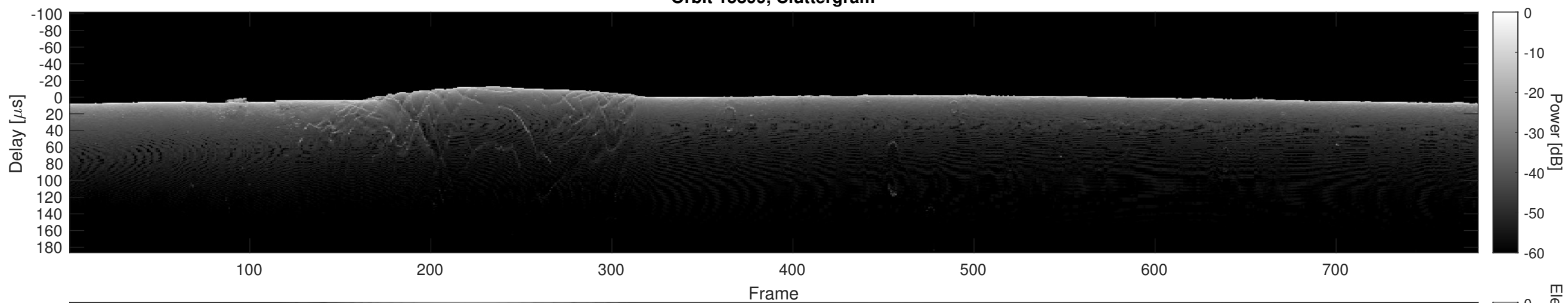
Orbit 15899, Cluttergram
