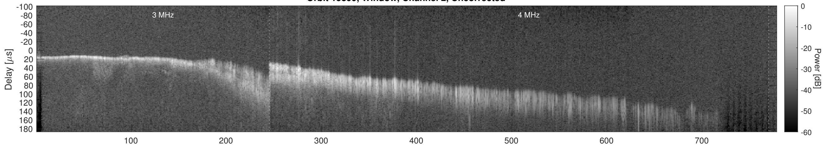
Orbit 15899, Window, Channel 2, Chapman
