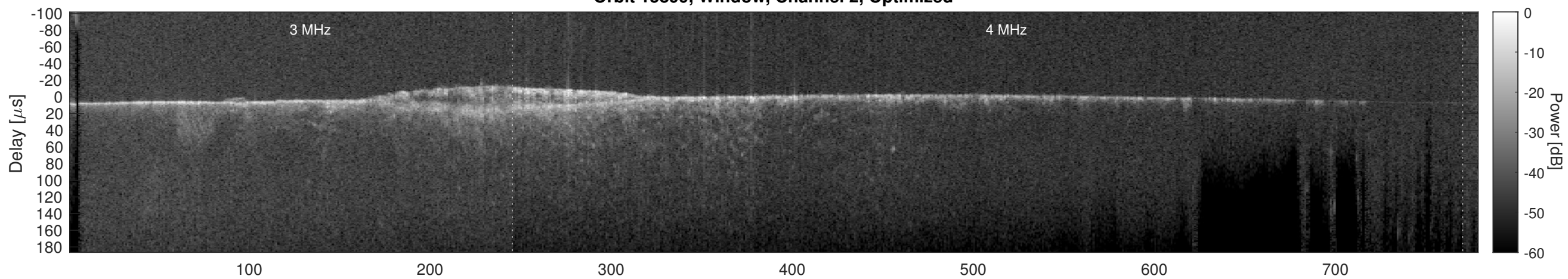
Orbit 15899, Cluttergram
