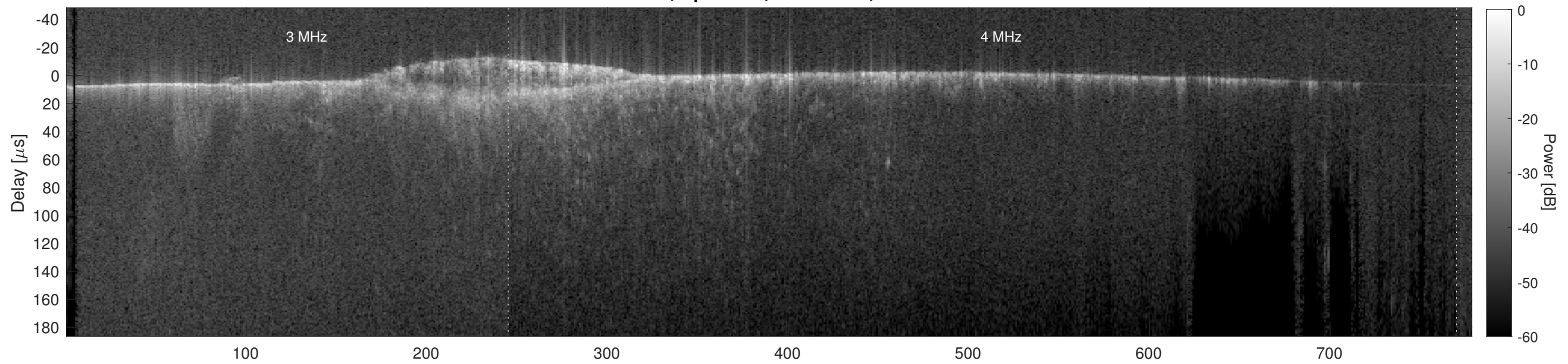
Orbit 15899, Cluttergram
