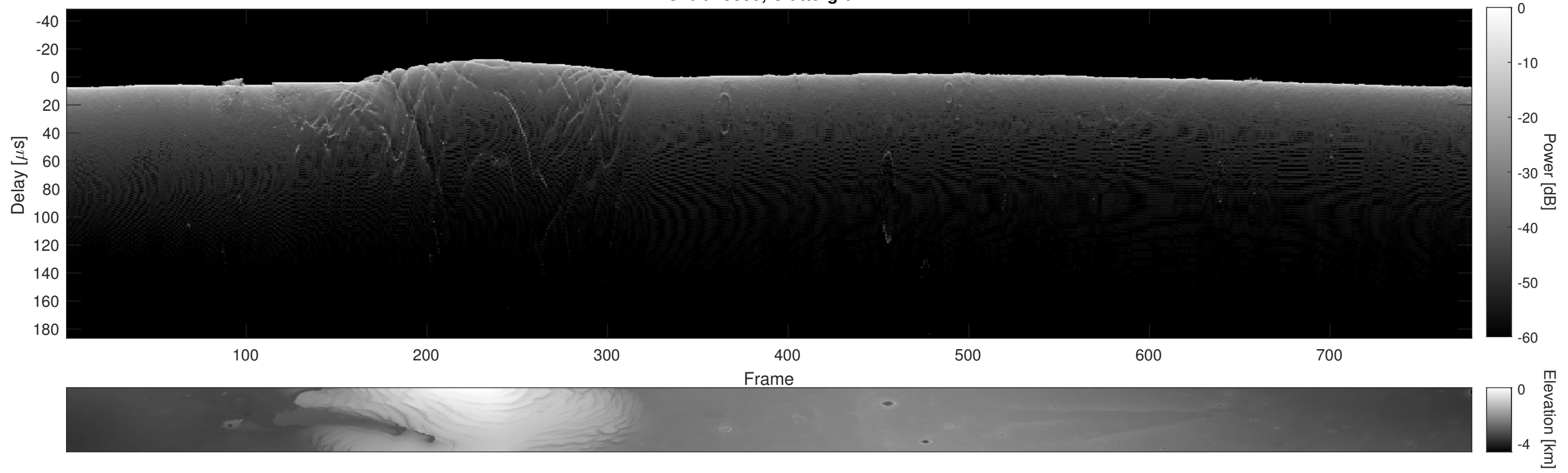
Orbit 15899, Cluttergram
