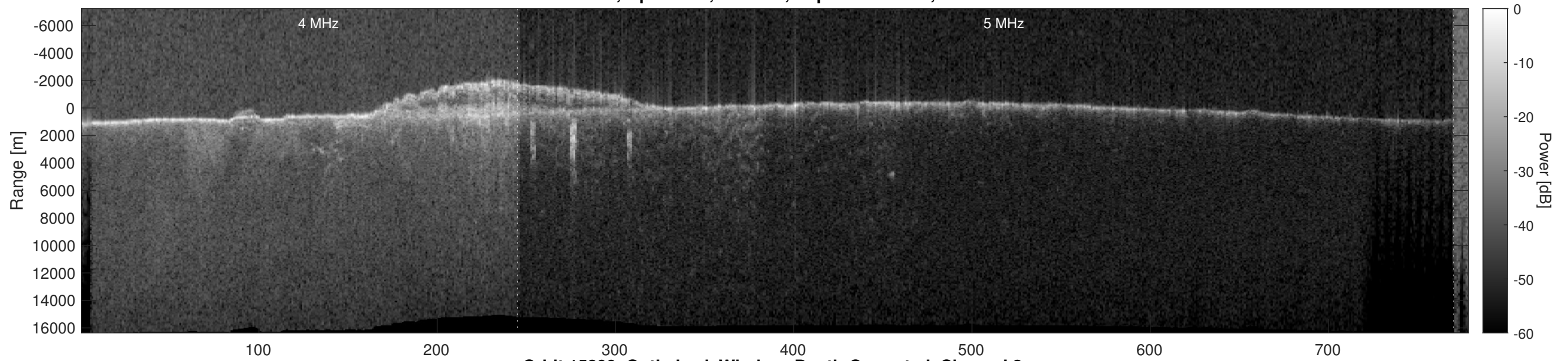
Orbit 15899, Optimized, Window, Depth-Corrected, Channel 2
