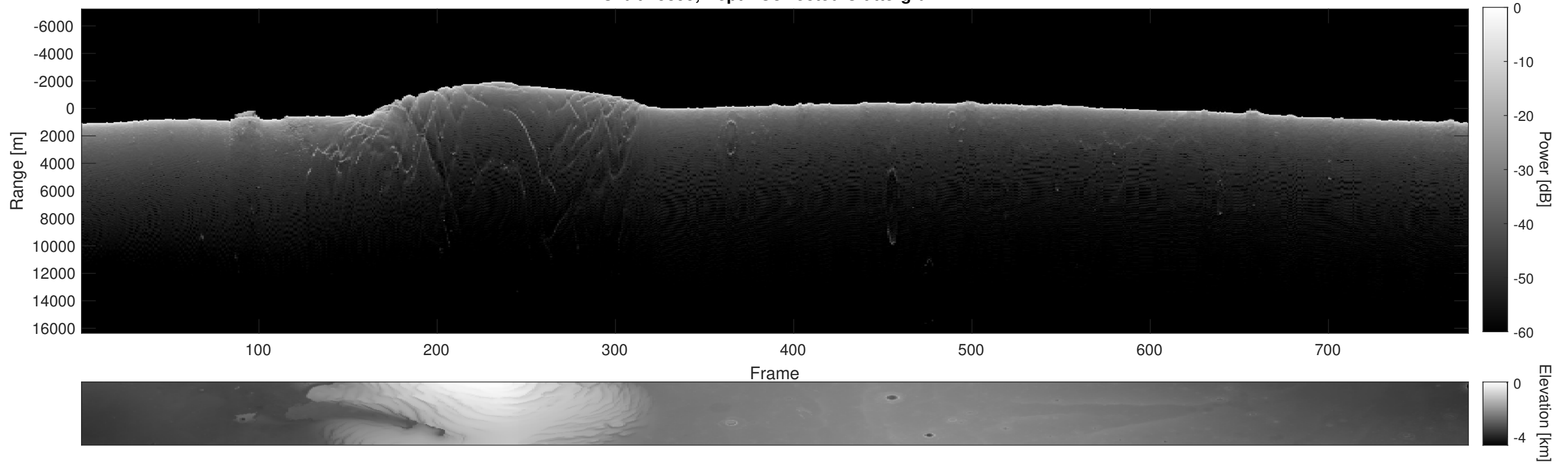
Orbit 15899, Depth-Corrected Cluttergram
