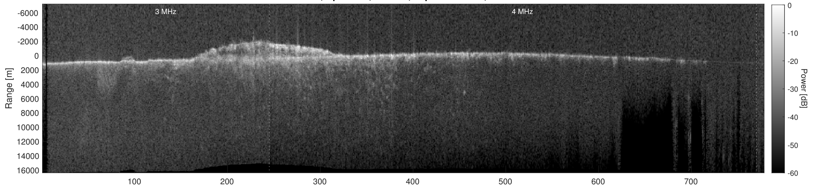
Orbit 15899, Depth-Corrected Cluttergram
