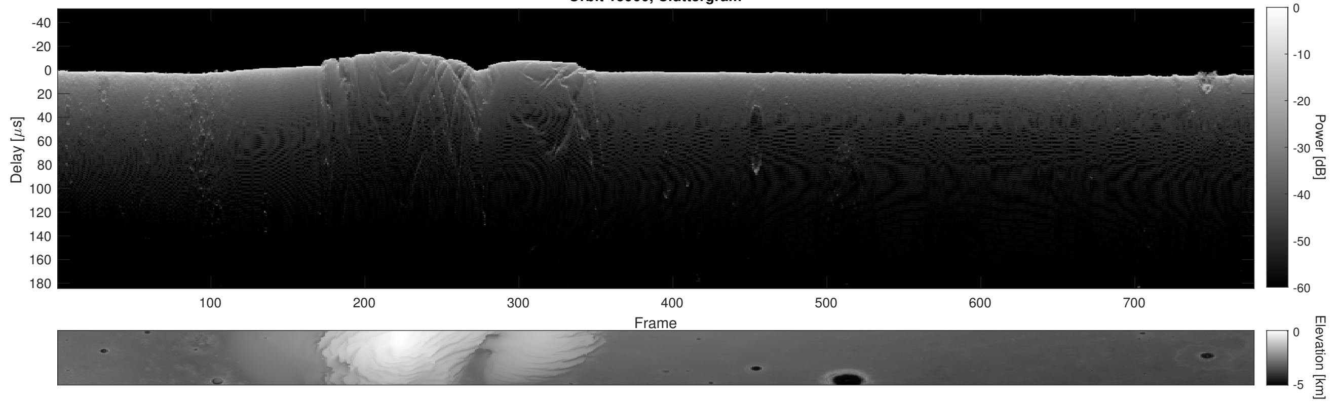
Orbit 15900, Cluttergram
