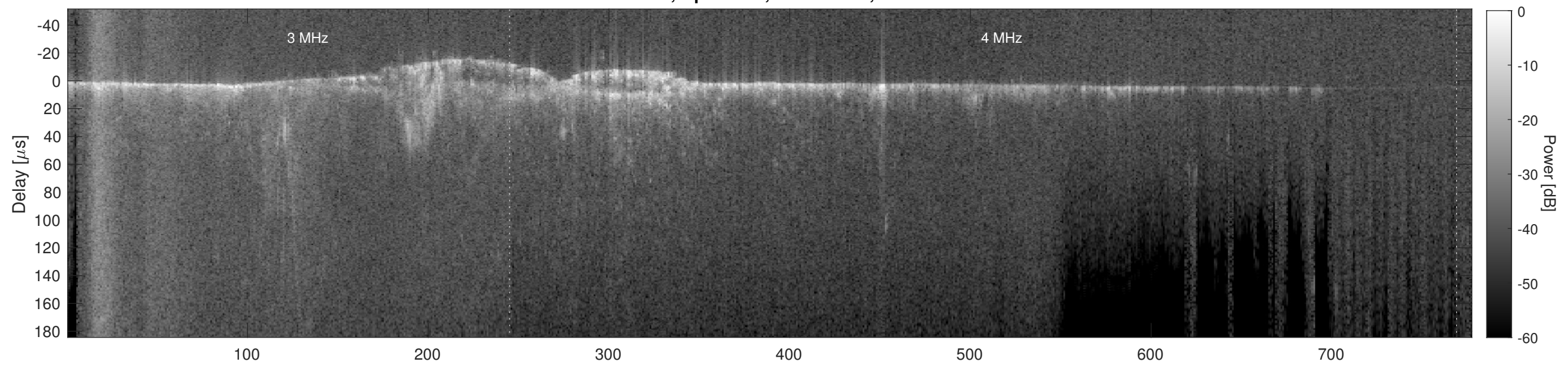
Orbit 15900, Cluttergram
