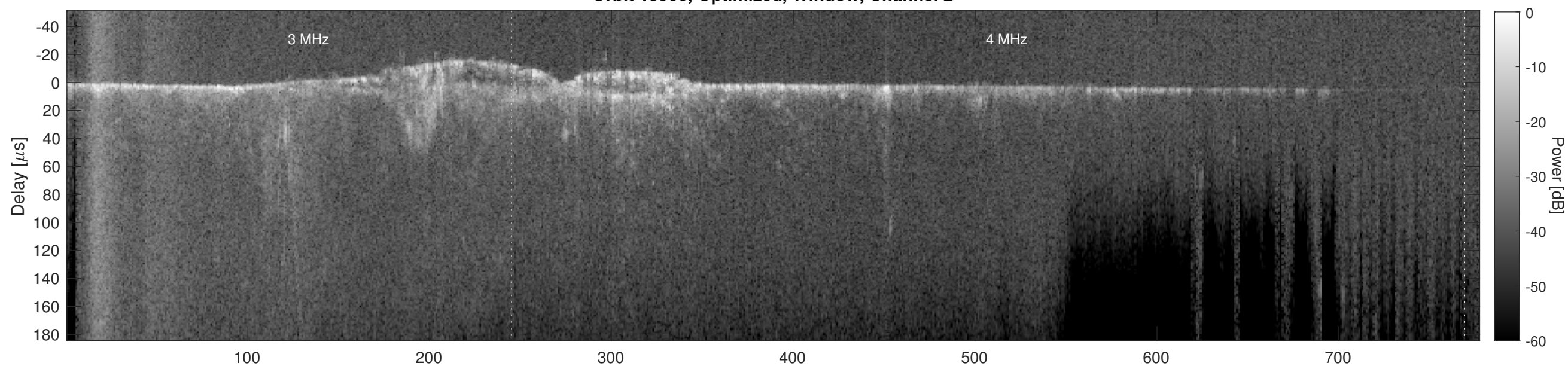
Orbit 15900, Cluttergram
