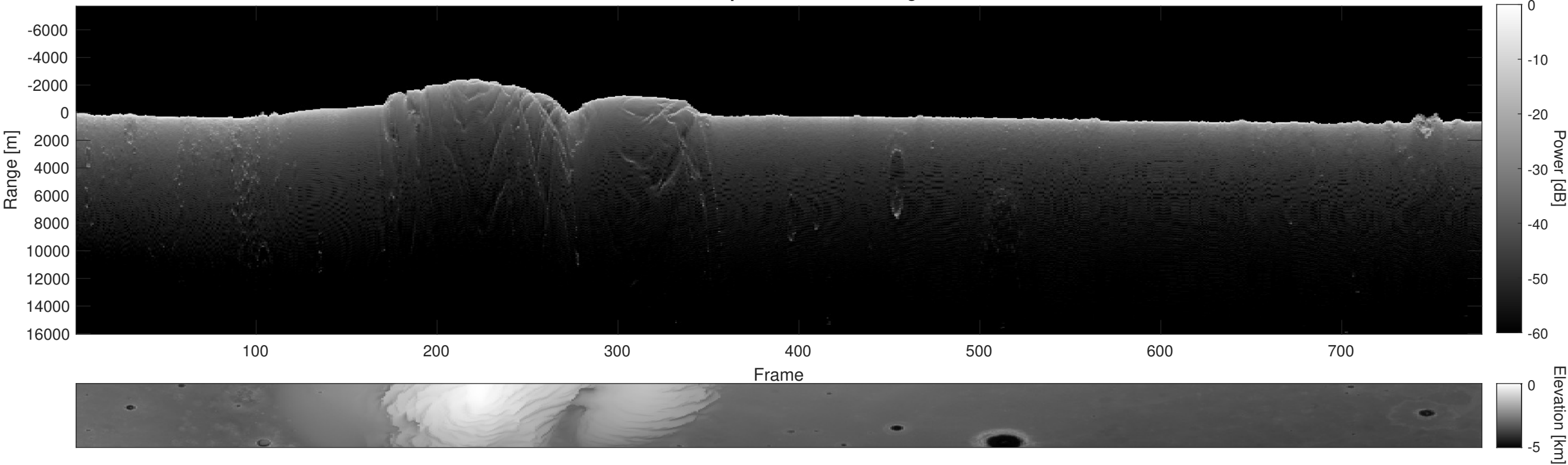
Orbit 15900, Depth-Corrected Cluttergram
