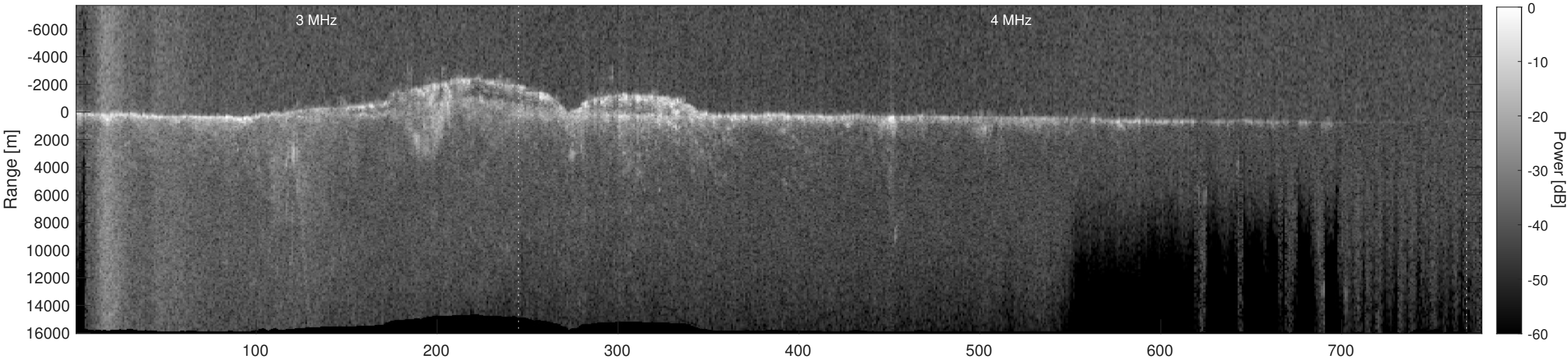
Orbit 15900, Depth-Corrected Cluttergram
