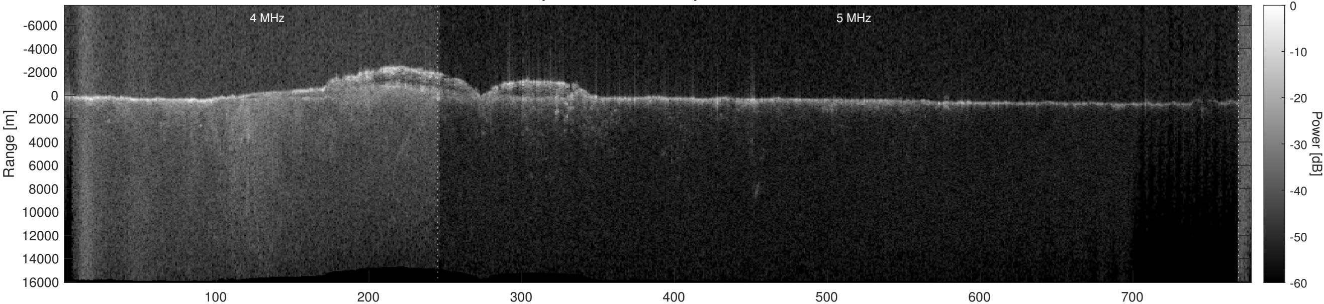
Orbit 15900, Optimized, Window, Depth-Corrected, Channel 2
