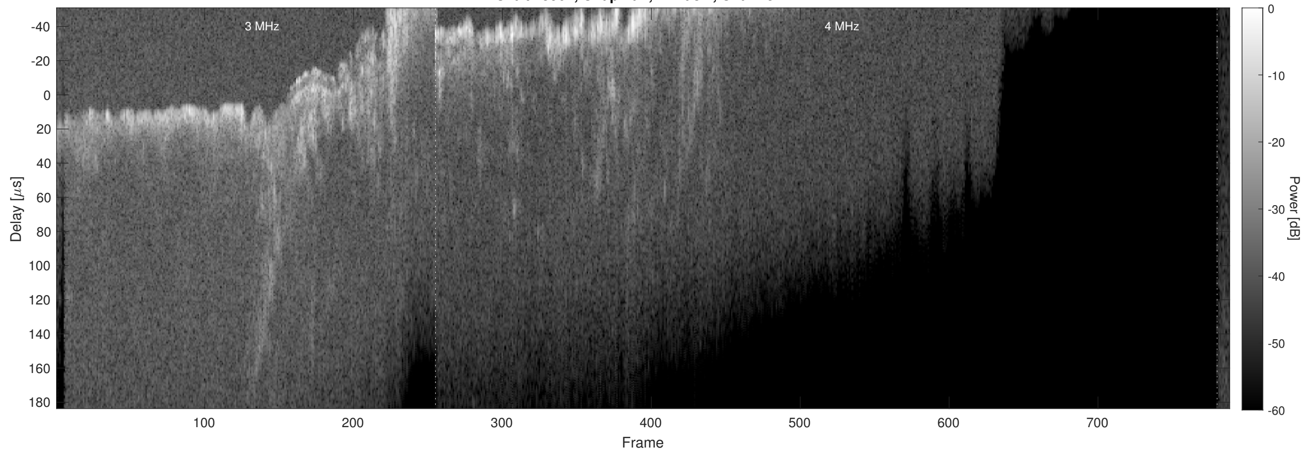
Orbit 15904, Chapman, Window, Channel 2
