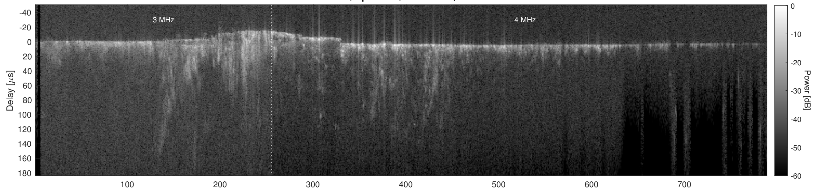
Orbit 15904, Cluttergram
