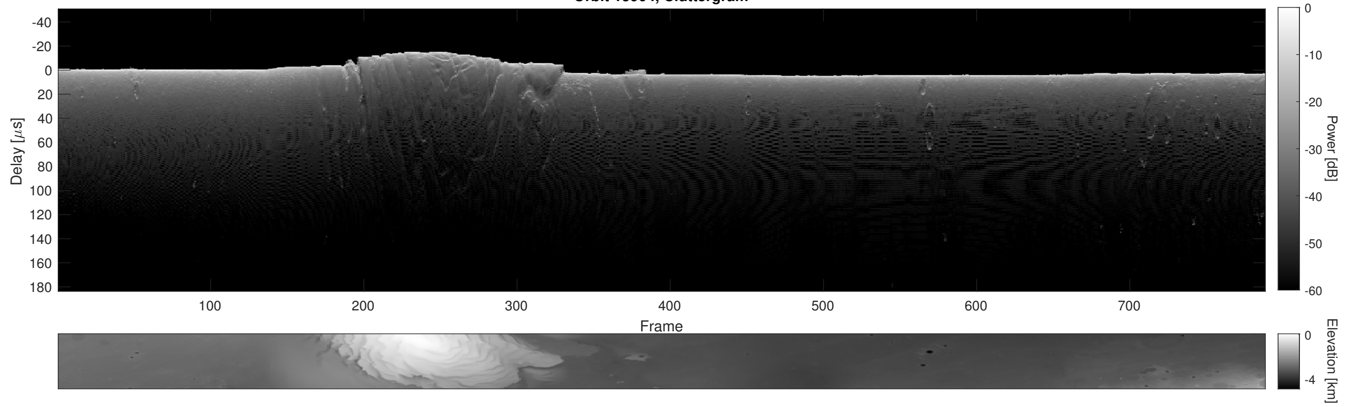
Orbit 15904, Cluttergram
