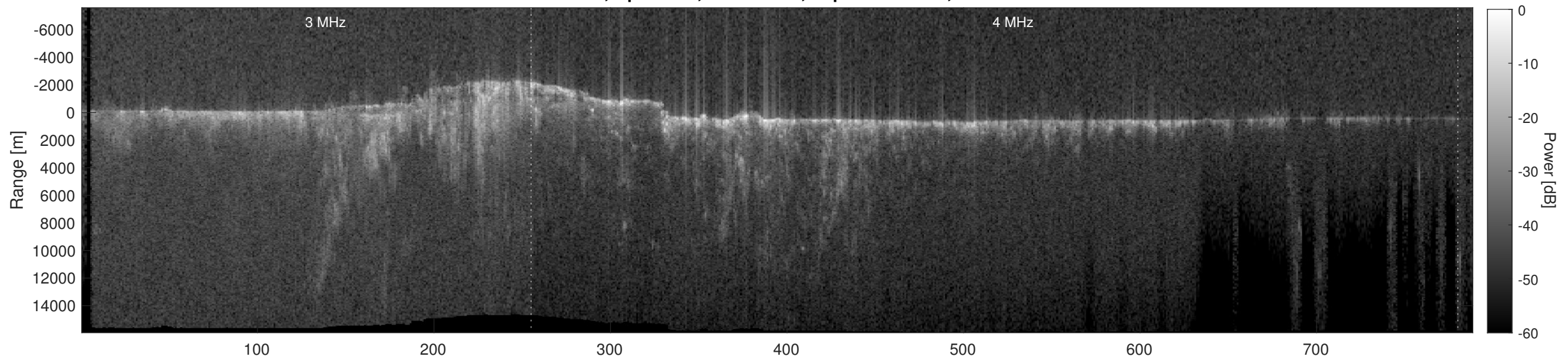
Orbit 15904, Depth-Corrected Cluttergram
