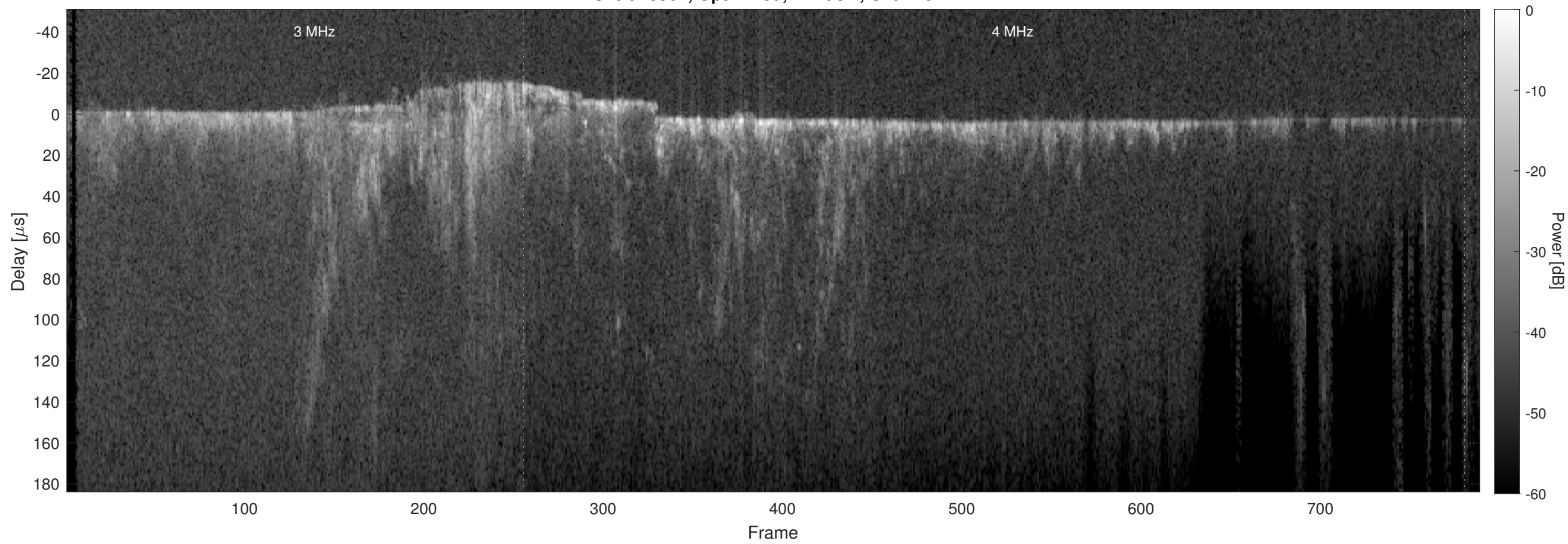
Orbit 15904, Optimized, Window, Channel 2
