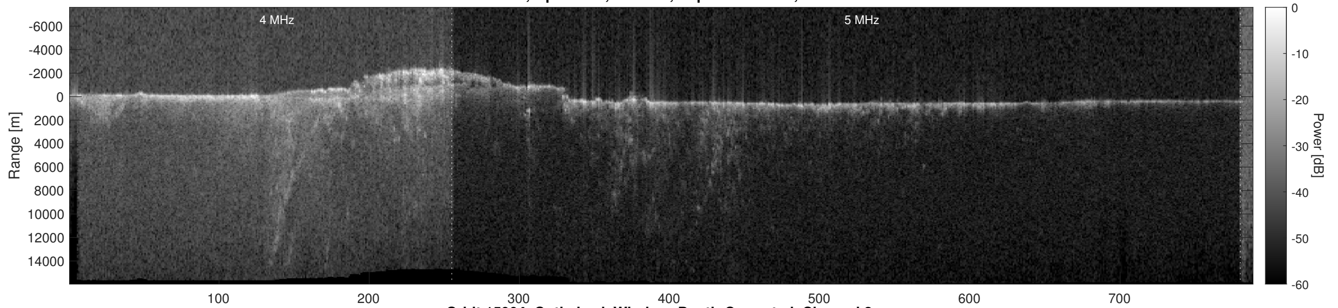
Orbit 15904, Optimized, Window, Depth-Corrected, Channel 2
