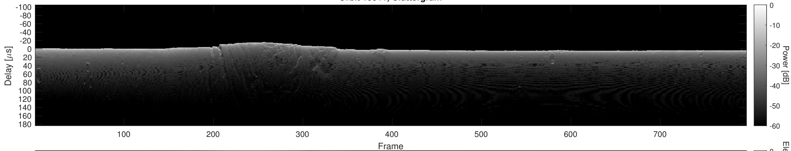
Orbit 15911, Cluttergram
