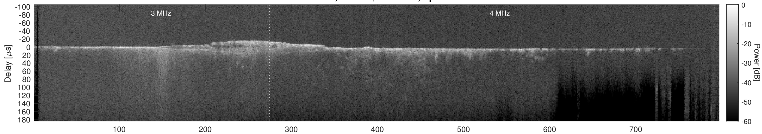
Orbit 15911, Cluttergram
