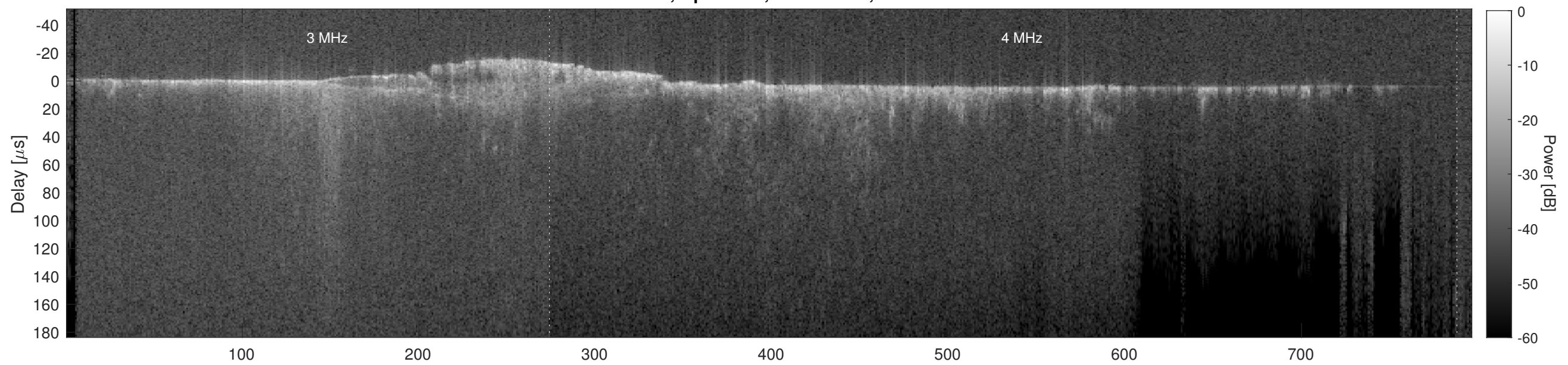
Orbit 15911, Cluttergram
