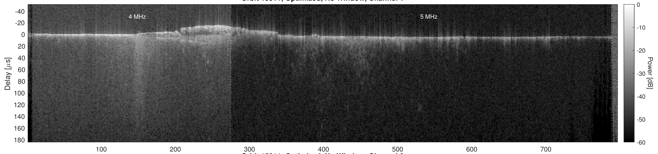
Orbit 15911, Optimized, No Window, Channel 2
