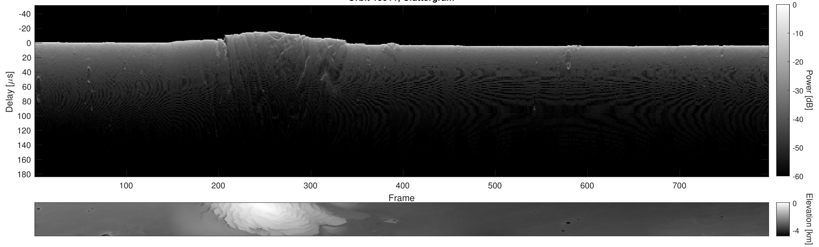
Orbit 15911, Cluttergram
