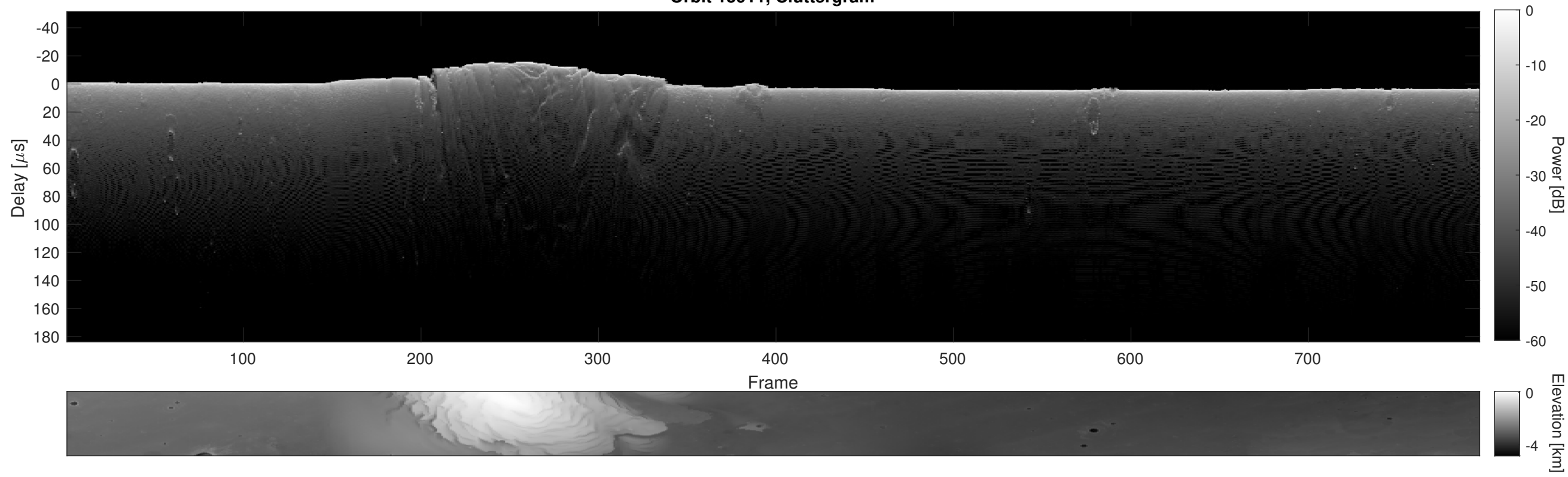
Orbit 15911, Cluttergram
