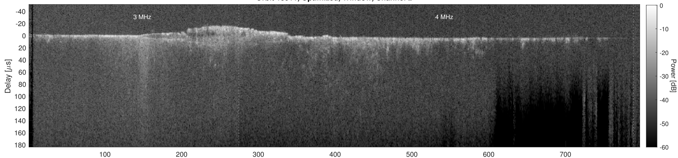
Orbit 15911, Cluttergram
