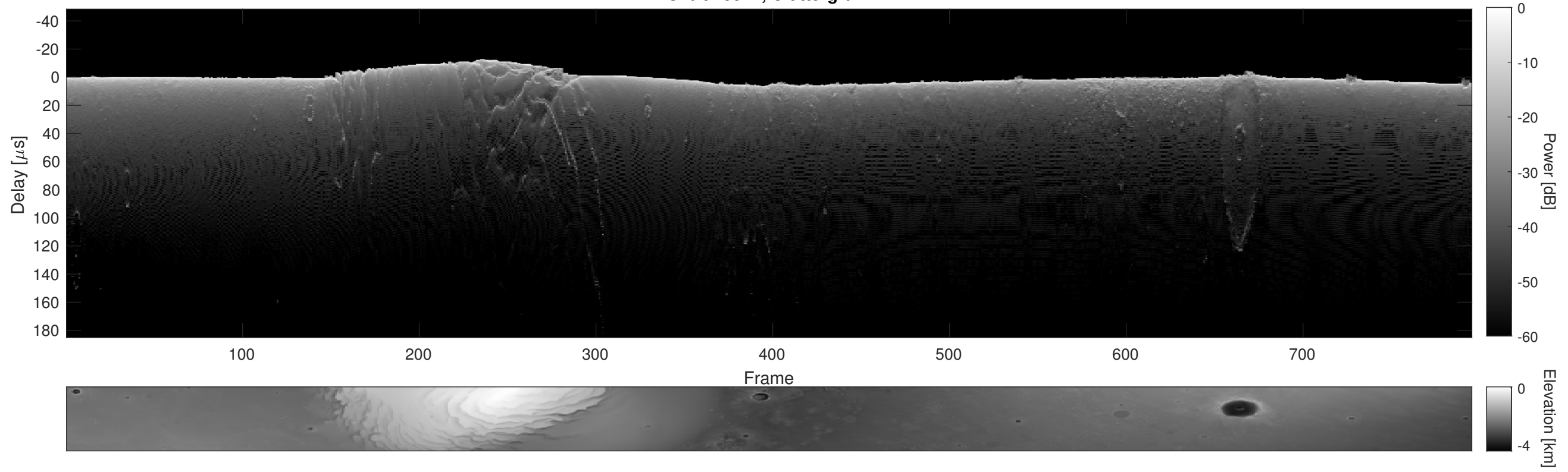
Orbit 15912, Cluttergram
