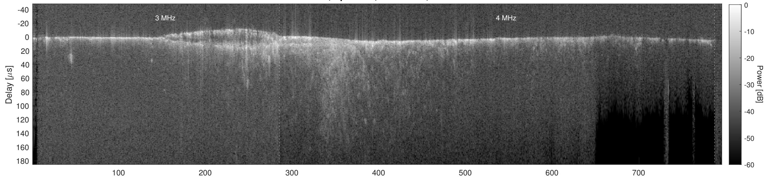
Orbit 15912, Cluttergram
