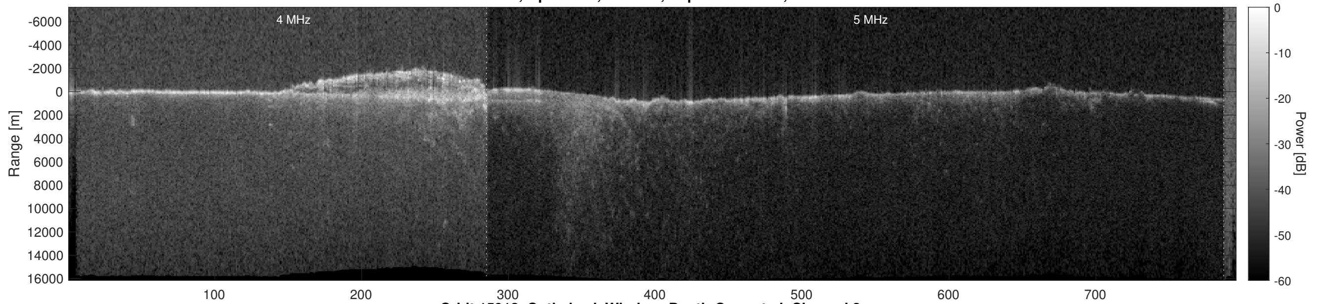
Orbit 15912, Optimized, Window, Depth-Corrected, Channel 2
