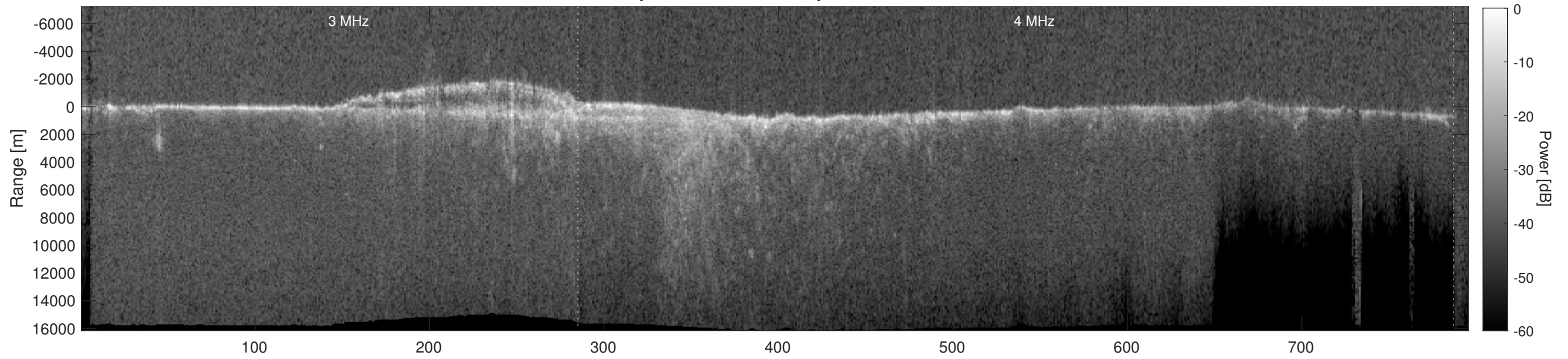
Orbit 15912, Depth-Corrected Cluttergram
