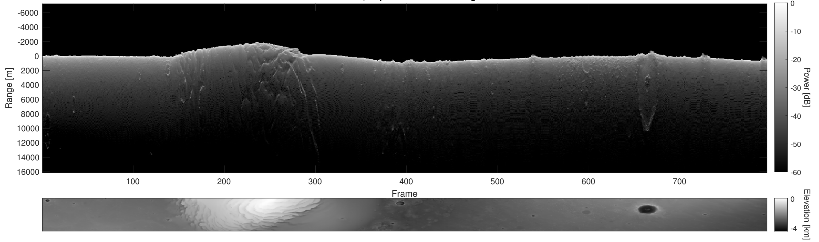
Orbit 15912, Depth-Corrected Cluttergram
