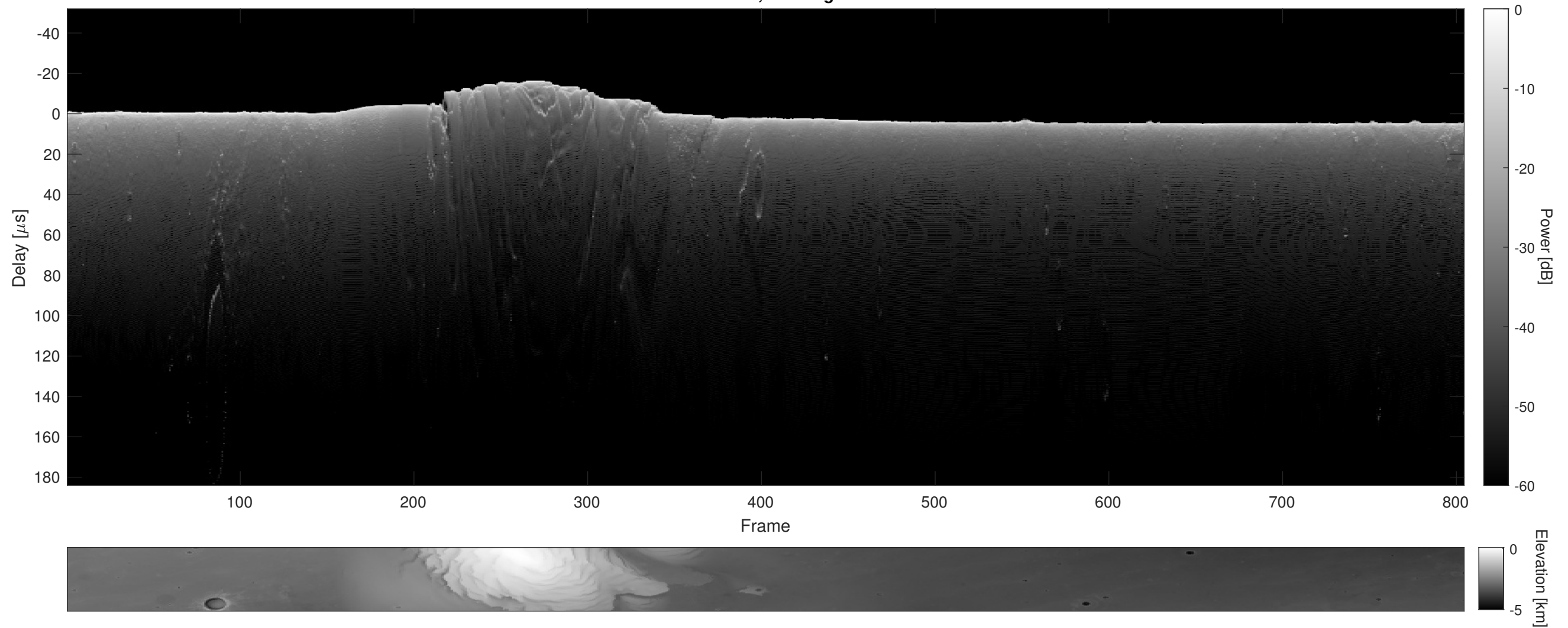
Orbit 15918, Cluttergram
