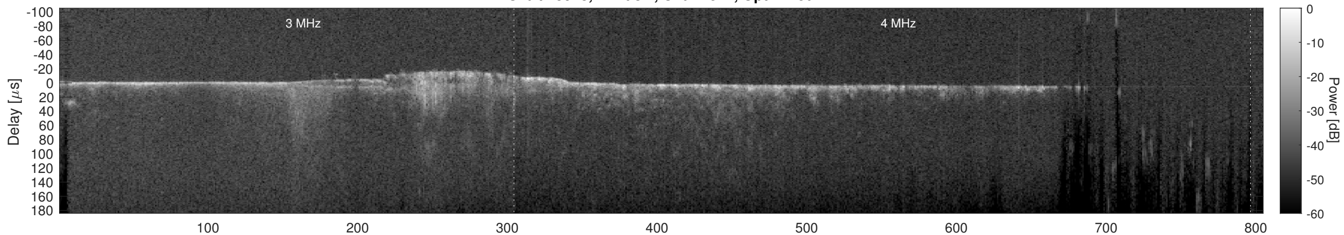
Orbit 15918, Cluttergram
