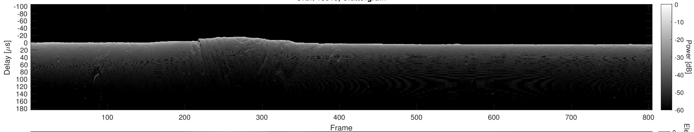
Orbit 15918, Cluttergram
