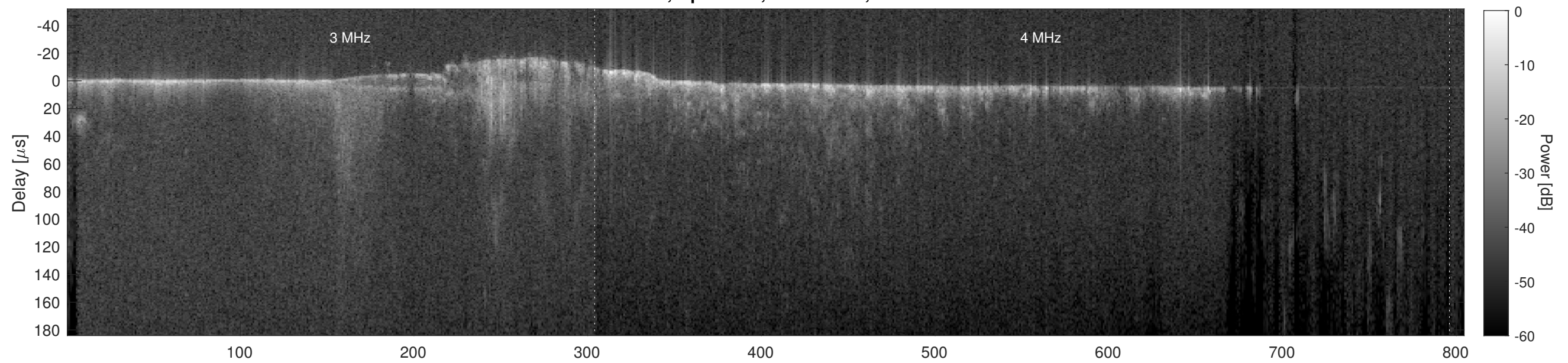
Orbit 15918, Cluttergram
