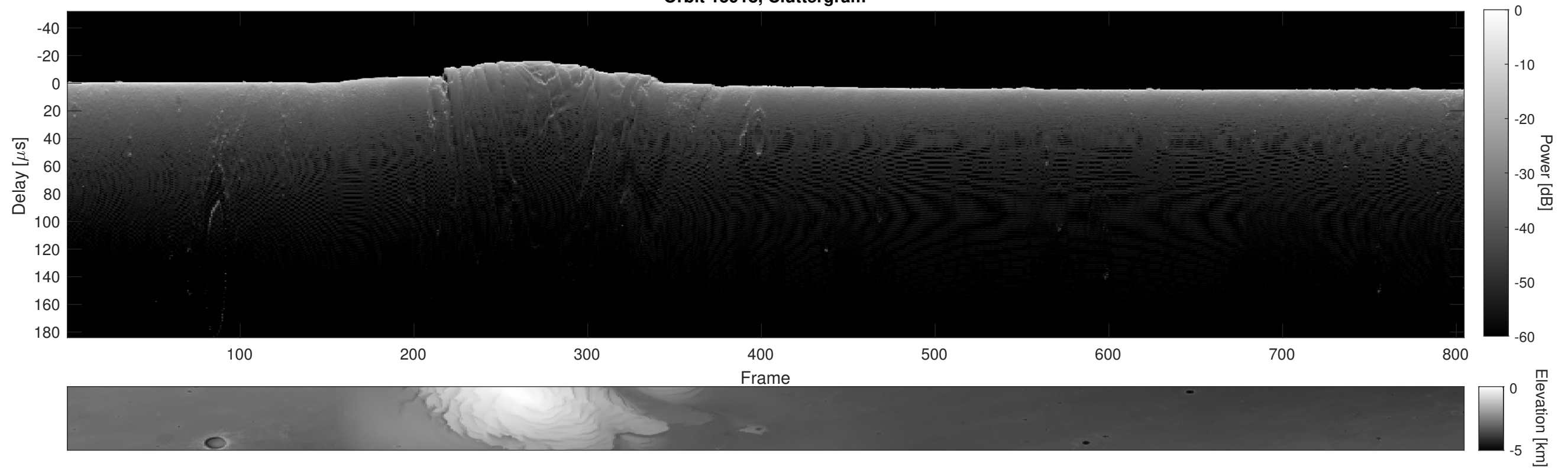
Orbit 15918, Cluttergram
