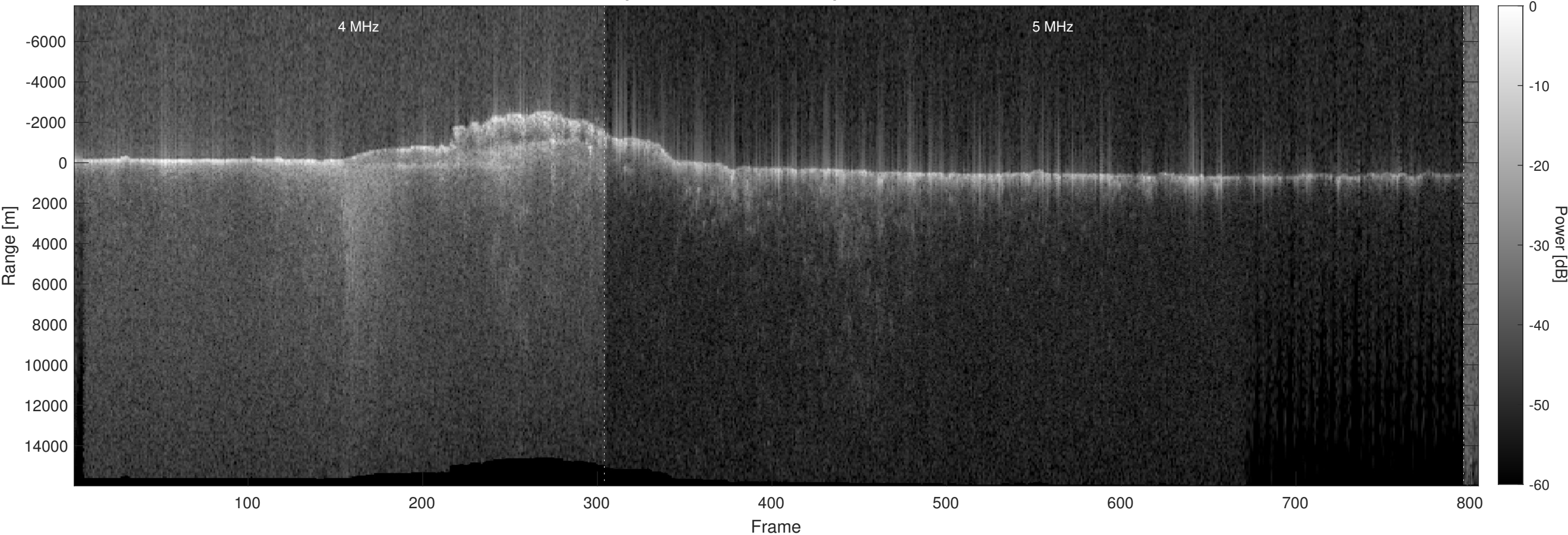
Orbit 15918, Optimized, No Window, Depth-Corrected, Channel 2
