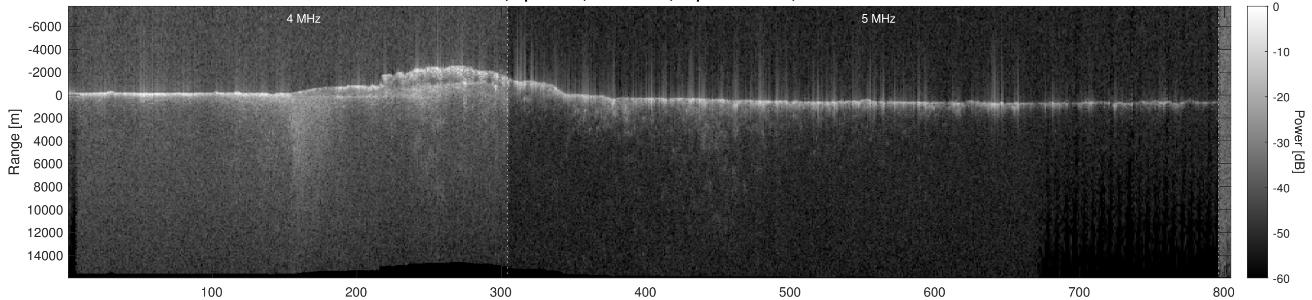
Orbit 15918, Optimized, No Window, Depth-Corrected, Channel 2
