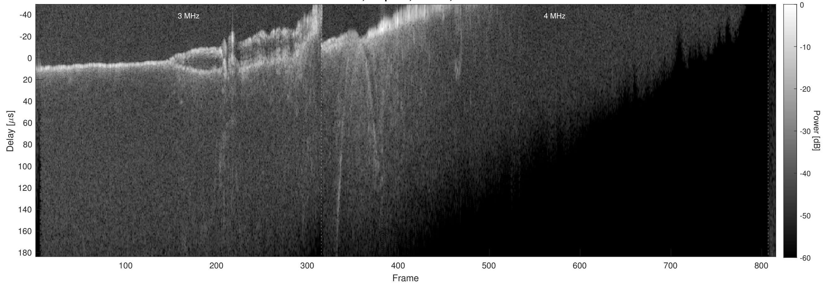
Orbit 15923, Chapman, Window, Channel 2
