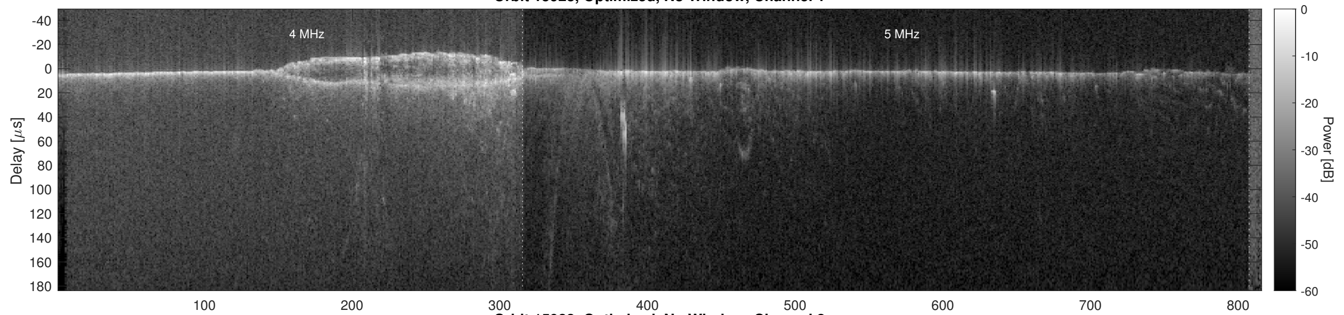
Orbit 15923, Optimized, No Window, Channel 2
