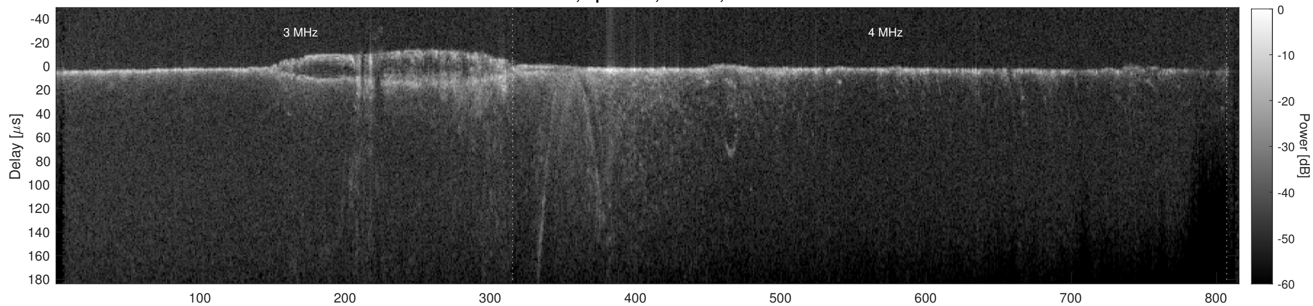
Orbit 15923, Cluttergram
