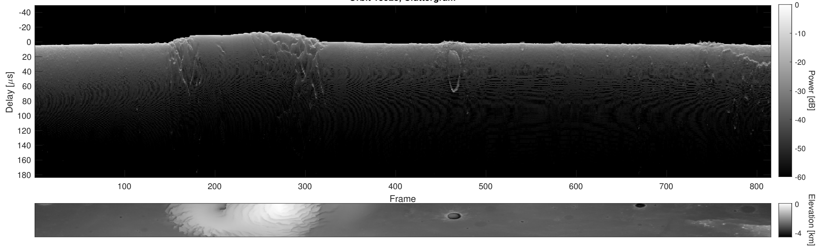
Orbit 15923, Cluttergram
