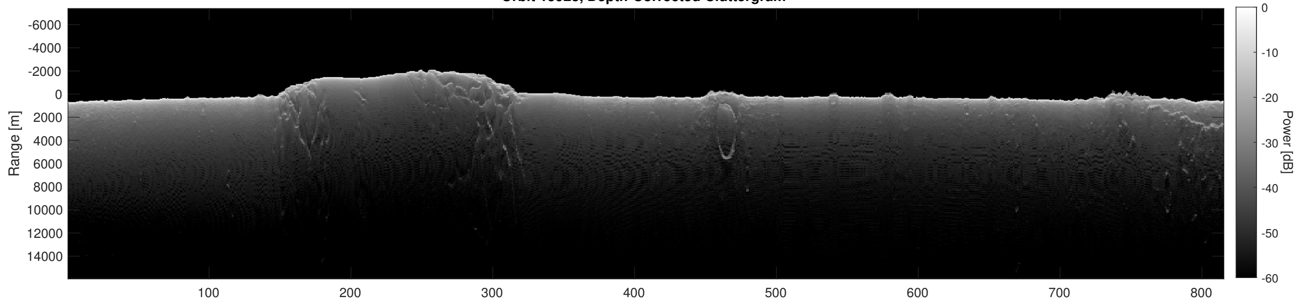
Orbit 15923, Depth-Corrected Cluttergram
