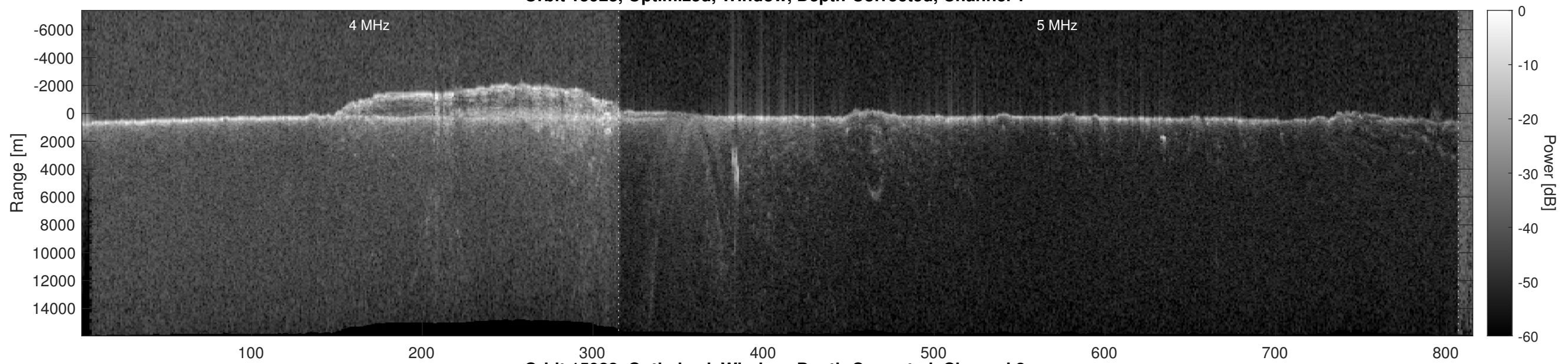
Orbit 15923, Optimized, Window, Depth-Corrected, Channel 2
