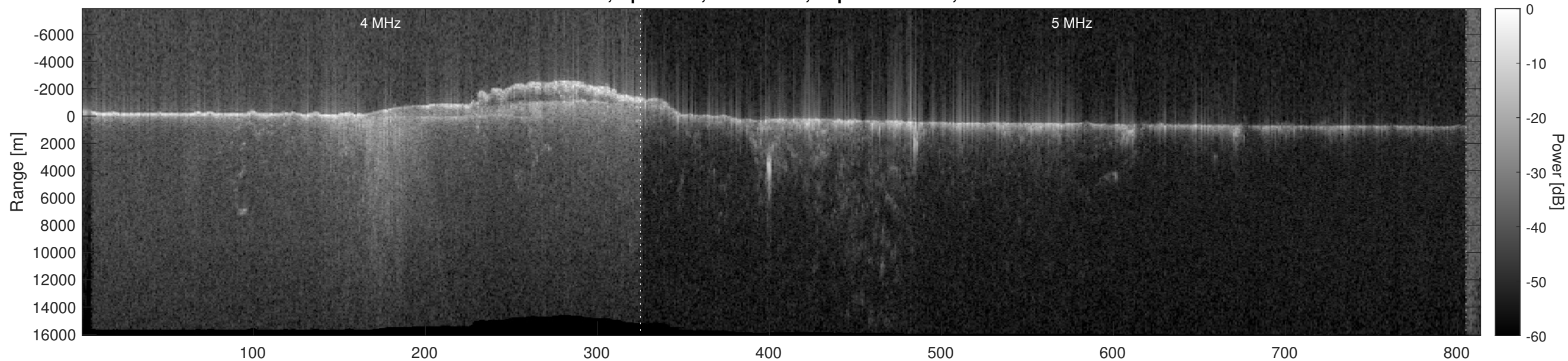
Orbit 15925, Optimized, No Window, Depth-Corrected, Channel 2
