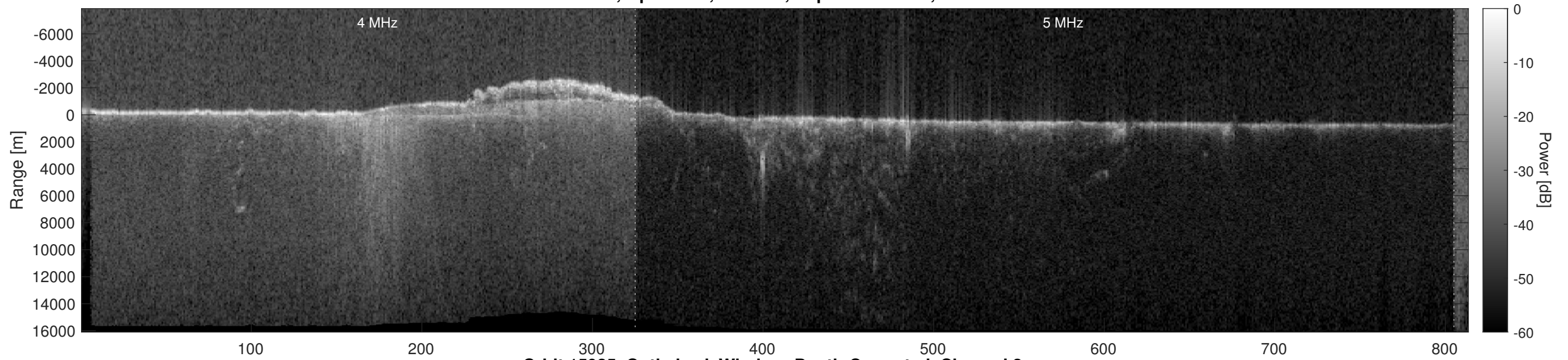
Orbit 15925, Optimized, Window, Depth-Corrected, Channel 2
