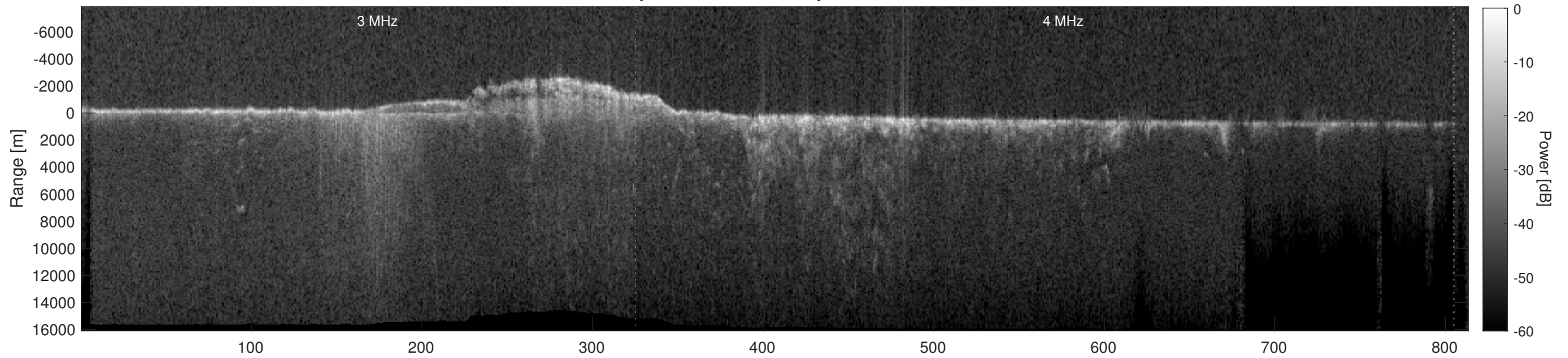
Orbit 15925, Depth-Corrected Cluttergram
