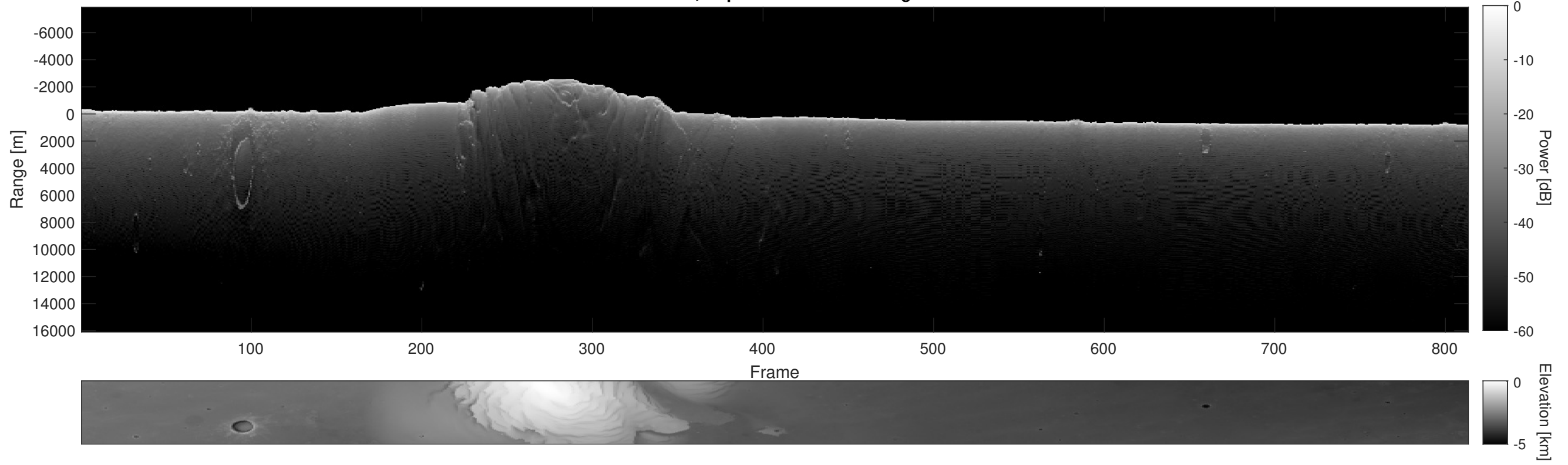
Orbit 15925, Depth-Corrected Cluttergram
