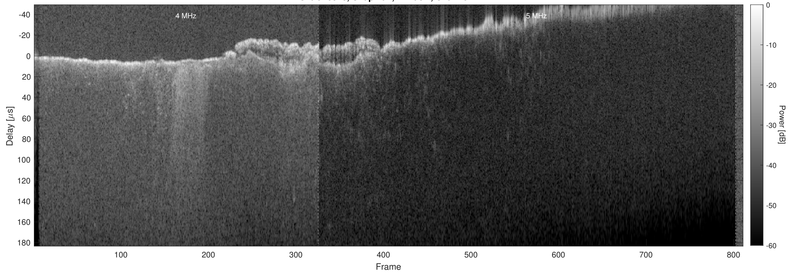
Orbit 15928, Chapman, Window, Channel 2
