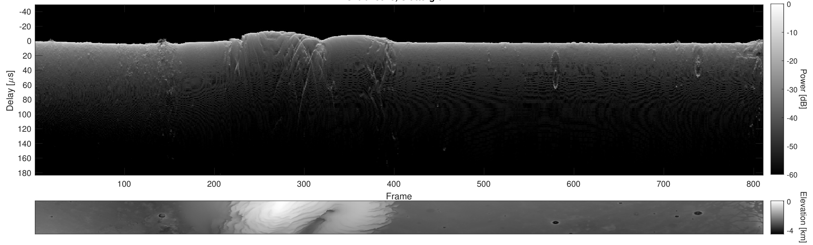
Orbit 15928, Cluttergram
