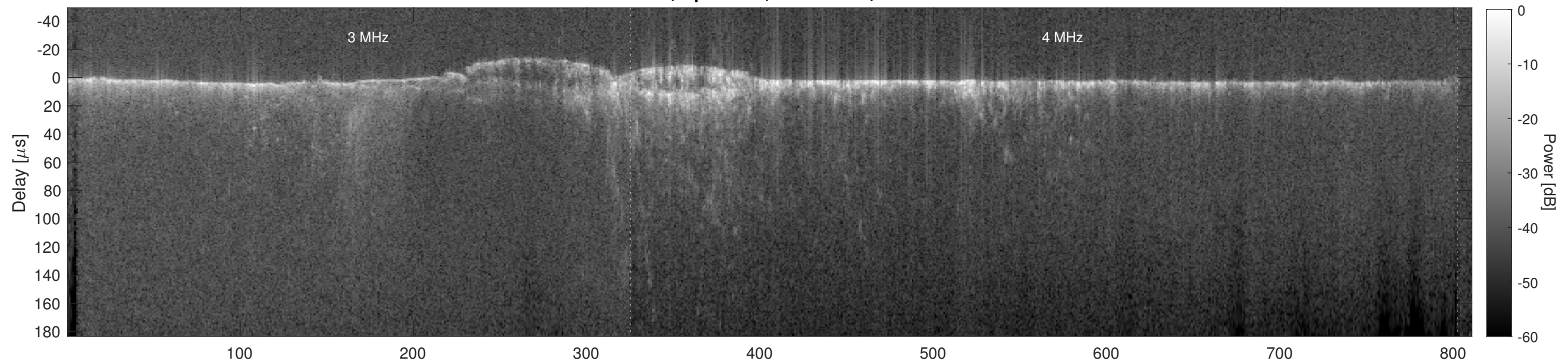
Orbit 15928, Cluttergram
