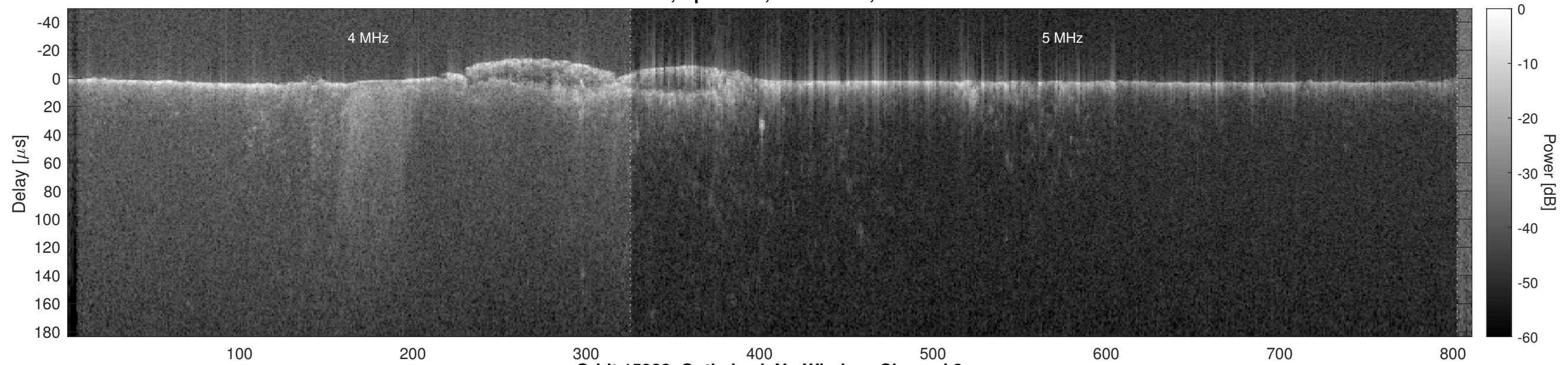
Orbit 15928, Optimized, No Window, Channel 2
