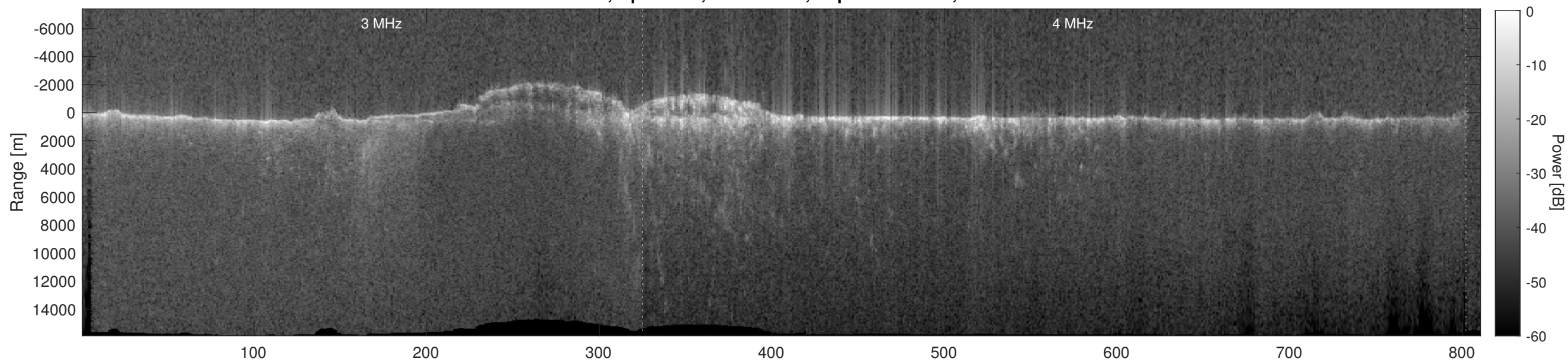
Orbit 15928, Depth-Corrected Cluttergram
