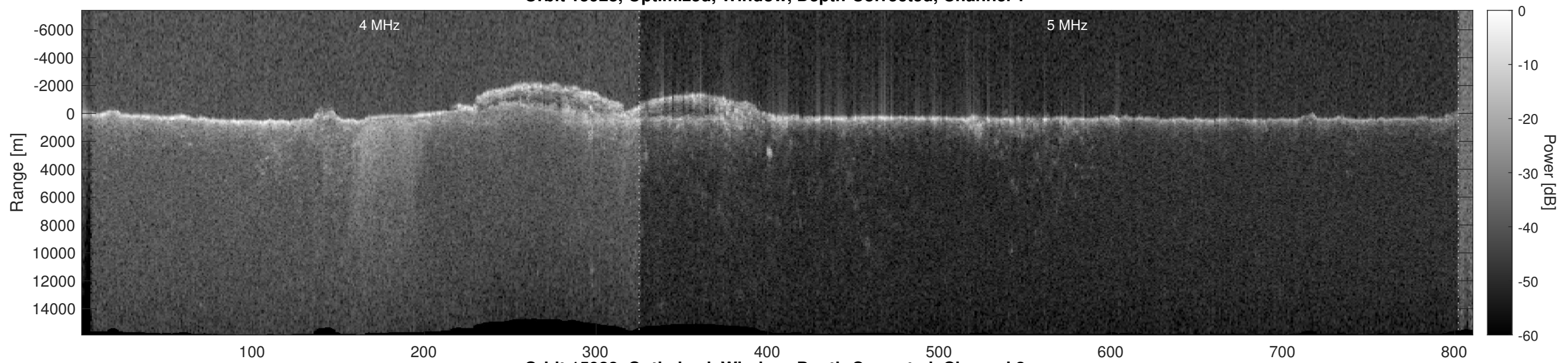
Orbit 15928, Optimized, Window, Depth-Corrected, Channel 2
