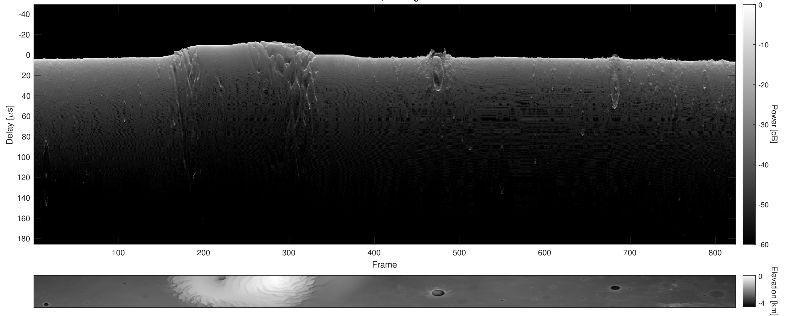
Orbit 15930, Cluttergram
