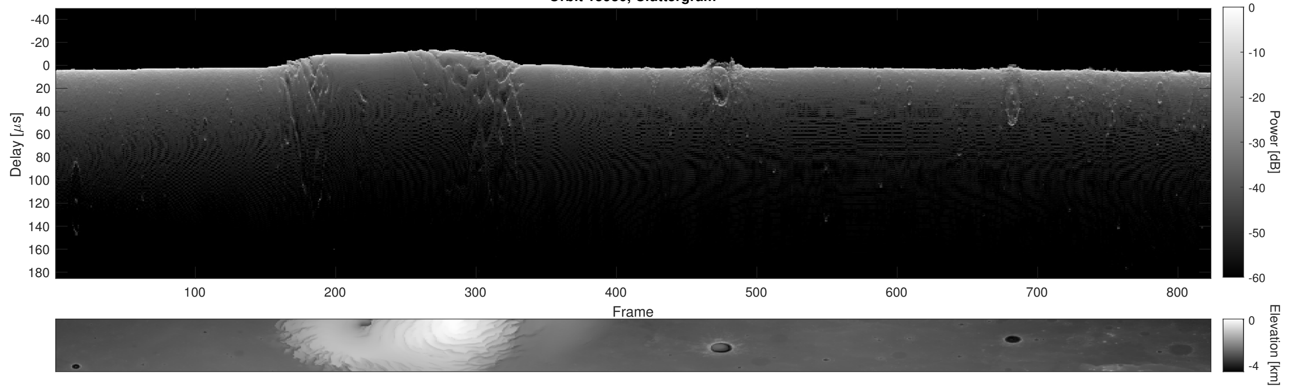
Orbit 15930, Cluttergram
