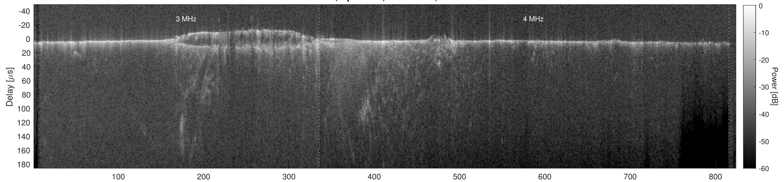
Orbit 15930, Cluttergram
