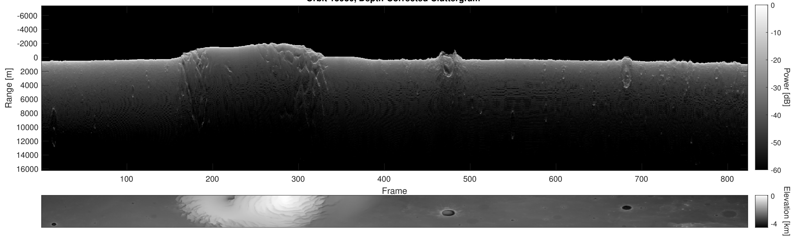
Orbit 15930, Depth-Corrected Cluttergram
