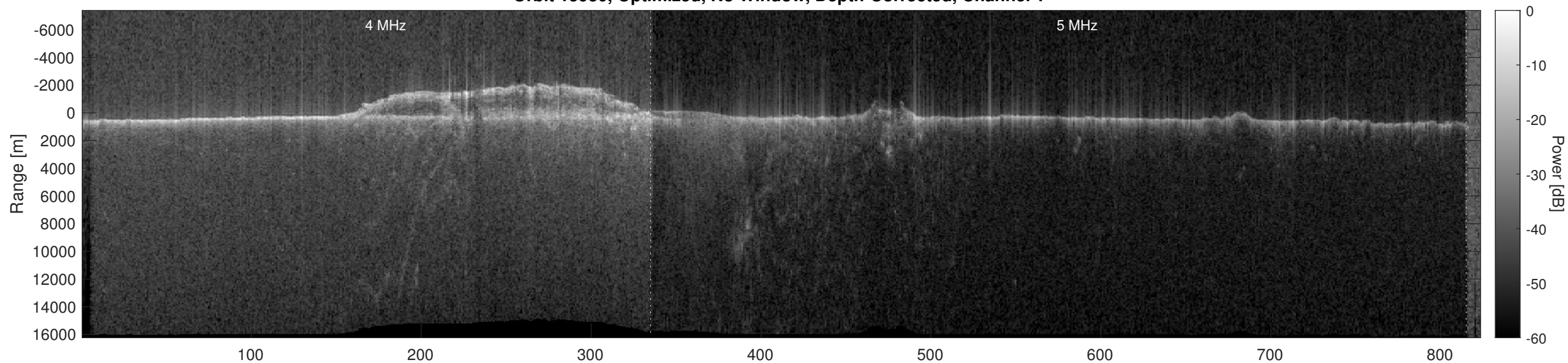
Orbit 15930, Optimized, No Window, Depth-Corrected, Channel 2
