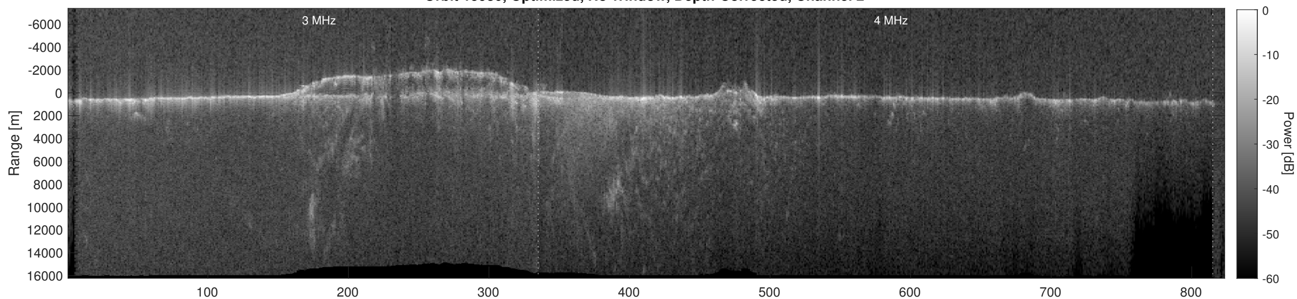
Orbit 15930, Depth-Corrected Cluttergram
