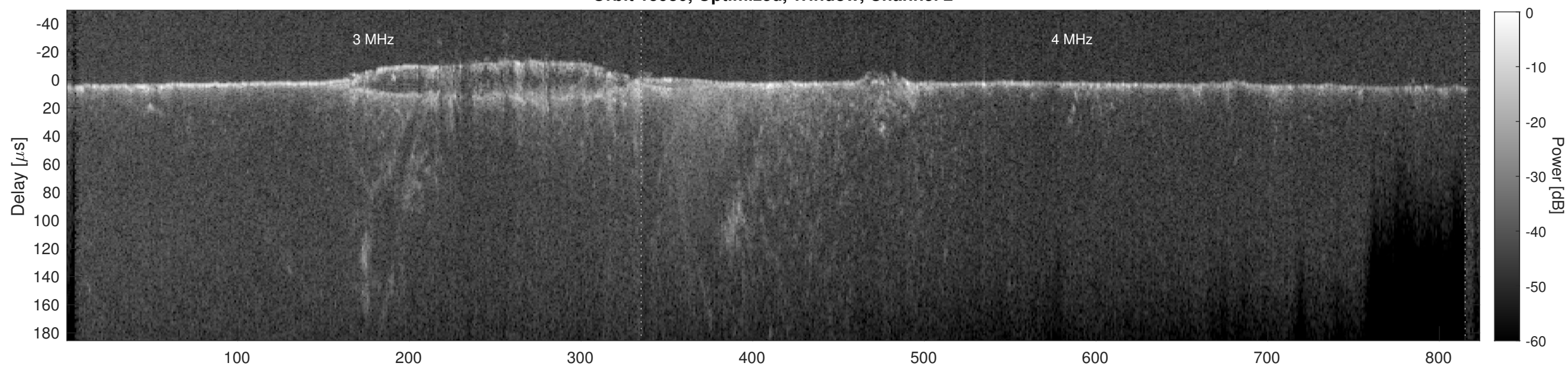
Orbit 15930, Cluttergram
