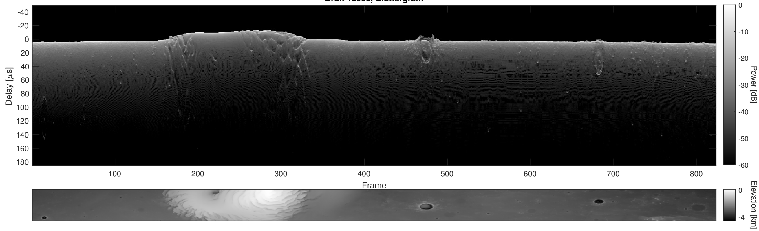
Orbit 15930, Cluttergram
